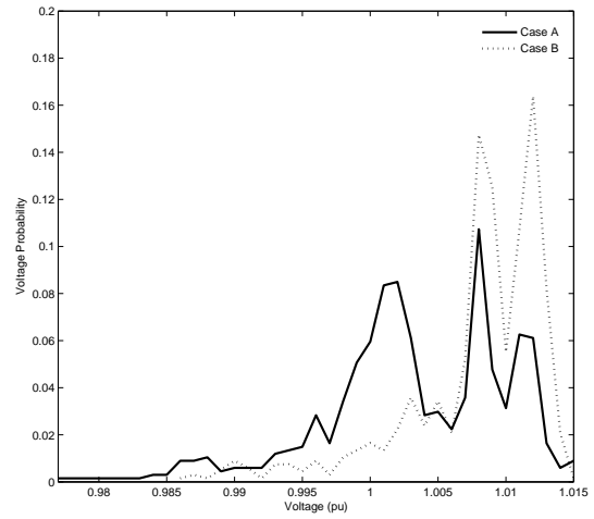
Fig. 3. Voltage PDF of rurally located 110kV bus in WR 4 for both Cases A and B. The PDF for Case B is shifted and contains more voltages operating at higher levels.
