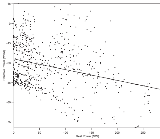
Fig. 5. The real power production from wind farms in WR 4 versus the reactive power production/consumption from the farms in the region for Case A.
