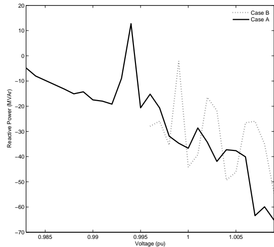
Fig. 8. The reactive power production for Cases A and B. Lower voltages are eliminated in Case B and the reactive power is not driven by wind power production.
