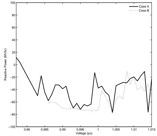
Fig. 4. Reactive power production of the wind turbines in Case A and B. Case B is more random indicating less dependence on wind power.
