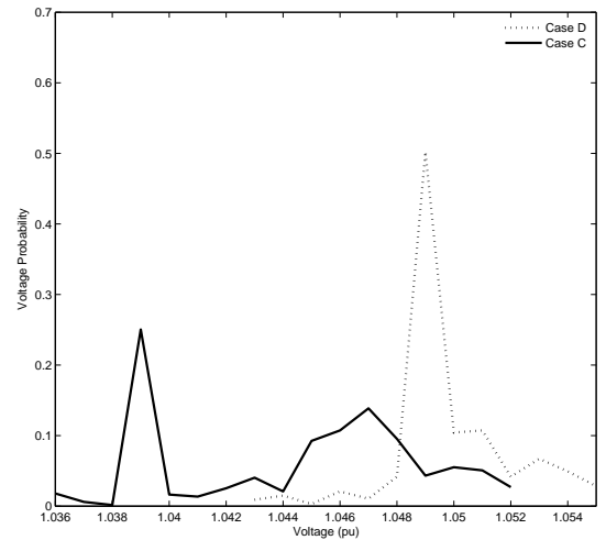
Fig. 10. The voltage PDF of a bus near Dublin for Cases C and D in WR 1. The probability of higher voltages increases in Case D, and show that a majority of the voltages lie at 1.049 pu.
