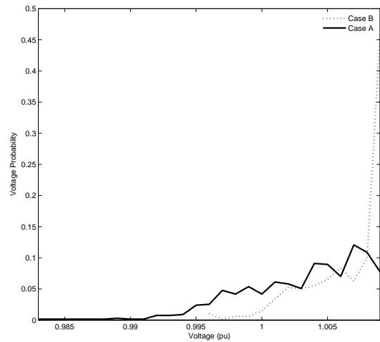
Fig. 7. Probability density function of the voltage of a 110kV bus in WR 1 plotted for Cases A and B. Case B shows a higher probability of increased voltages.
