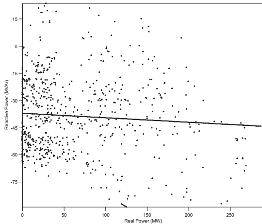
Fig. 6. The same P vs. Q plot except for Case B. Less slope in the linear regression indicates less dependence on real power.
