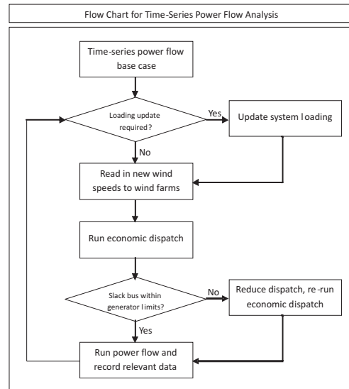
Fig. 2. Methodology used for time-series power flow analysis for one-week (672 power flows at 15-minute intervals) in SNV and WP loading scenarios.
