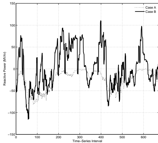
Fig. 11. The change in reactive power consumption over a one week period in the SNV between Case A and Case B.
