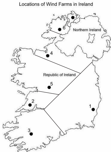
Fig. 1. Locations of the seven wind farms used in this study and the corresponding wind region divisions. Existing and future farms were mapped back to the nearest location.
