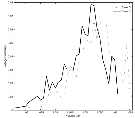
Fig. 9. The voltage PDF of the rurally located bus in WR 4 plotted for the two control cases. Voltages shift toward higher values as more terminal voltage control is enabled.
