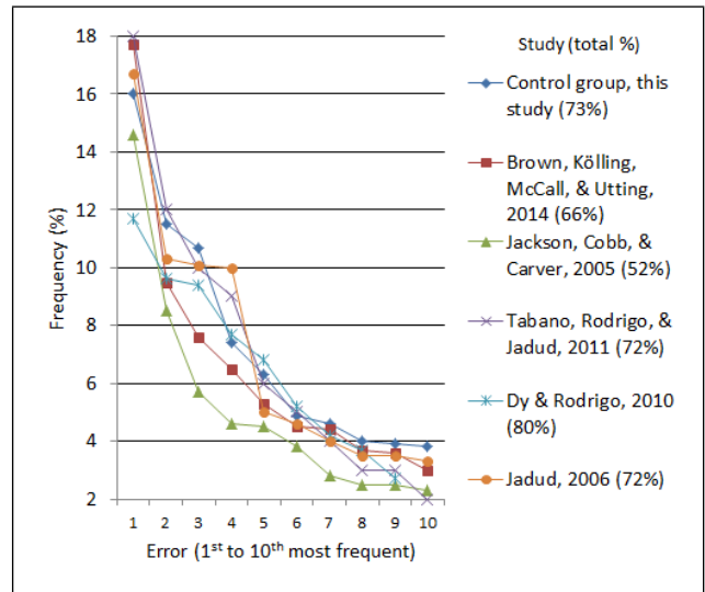
Figure 2: Frequency of the 10 most frequent compiler error messages from six studies.
