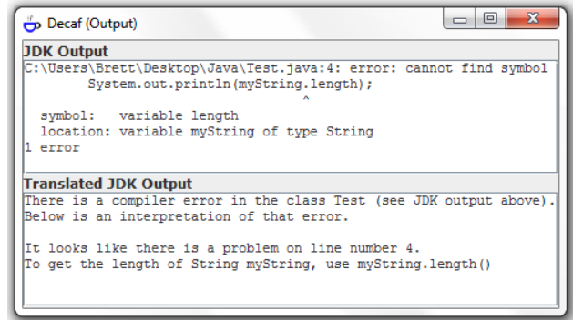
Figure 1: Decaf error window displaying an enhanced compiler error message resulting from incorrectly calling the length() method of the String class which generated a cannot find symbol javac error message.
