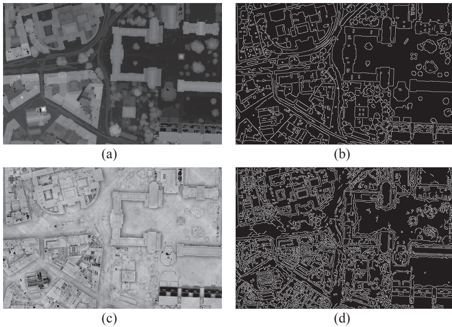
Figure 14: Edge detection comparison: (a) an elevation image; (b) detected edges for the elevation image in part (a); (c) an occlusion image; (d) detected edges for the occlusion image in part (c). Pixel dimensions are \Delta x = \Delta y = 0.50 \text{ m} .
