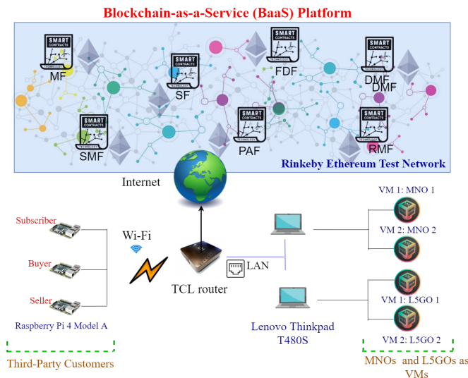
Fig. 14: Implementation Testbed.
