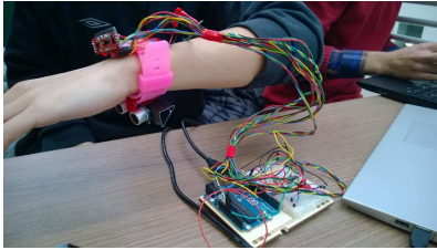
Figure 4. Our prototype device for exploring our proposed interactions. The IR sensors for detecting gestures on the back of the hand can be seen on the top left of the strap. On the underside of the strap are the ultrasound speakers and microphones.
