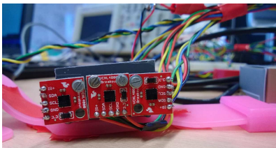
Figure 5. Three infrared sensors were placed on the side of the device to triangulate interaction data above the hand. By including three sensors, we can mitigate against sensor occlusion during interaction.
