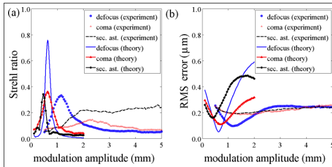
Fig. 3. Effect of modulation amplitude on wavefront sensing accuracy in the experiments and theoretical predictions at \text{SNR} = \infty in terms of (a) Strehl ratio and (b) RMS error.
