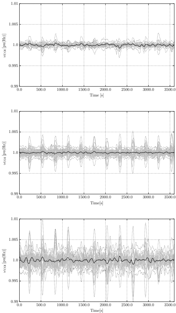
Fig. 4: Frequency \omega_{COI} with 2 (upper panel); 6 (middle panel); and 12 (lower panel) MGs. The grey lines represent each realization, the black thick line represents the average of the process, while the dotted line represents the average \pm 3 times the standard deviation.
