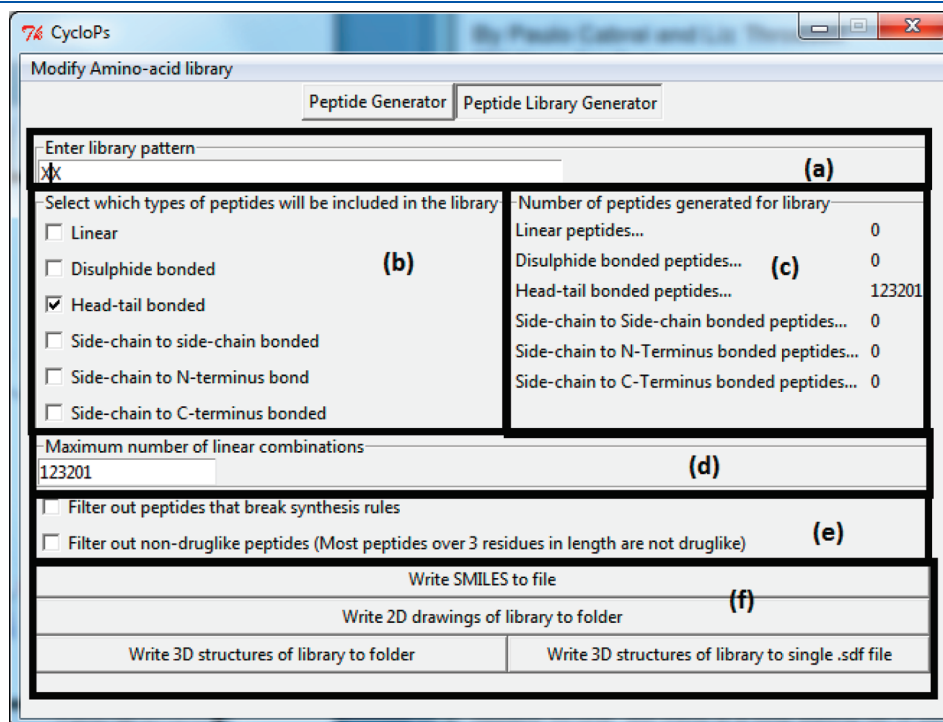
Figure 5. CycloPs library generation interface. (a) Library pattern entry box. (b) Library included constraint selection pane. (c) Library peptide count information pane. (d) Maximum number of linear combinations: this gives a quick estimate of the library size. If this is above 1 000 000 peptides, the counts for each constraint will not be generated due to time constraints, as each sequence is generated and tested individually for each constraint. (e) Library filtering options. (f) Library output options.
