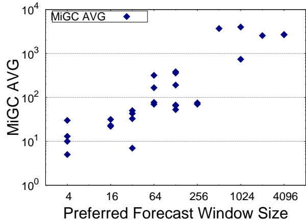
Fig. 6. Preferred FWS vs. MiGC AVG
