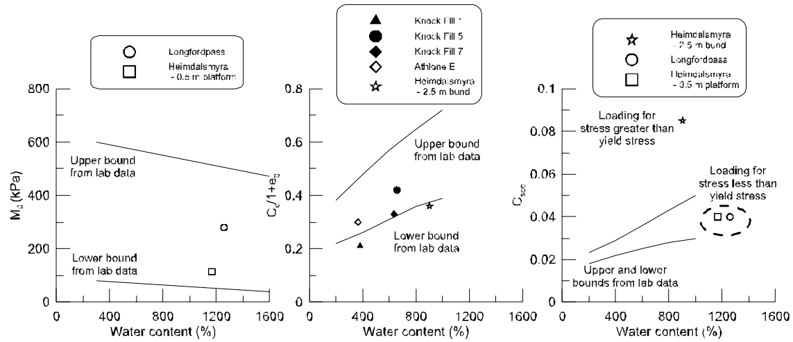
Fig 17. Parameters backanalysed from case histories (a) M_0 , (b) C_c/(1+e_0) and (c) C_{sec}
