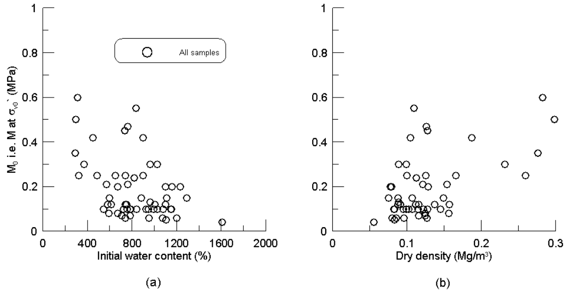
Fig. 6. Constrained modulus M_0 , i.e. M at \sigma'_{v0} versus (a) water content and (b) dry density
