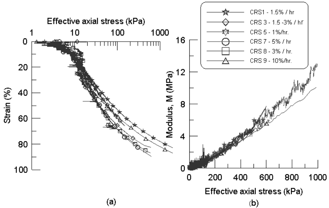
Fig. 5. Constant rate of strain (CRS) tests West Mayo site (a) \log \sigma'_v \text{ v } \epsilon , (b) \sigma'_v \text{ v } M
