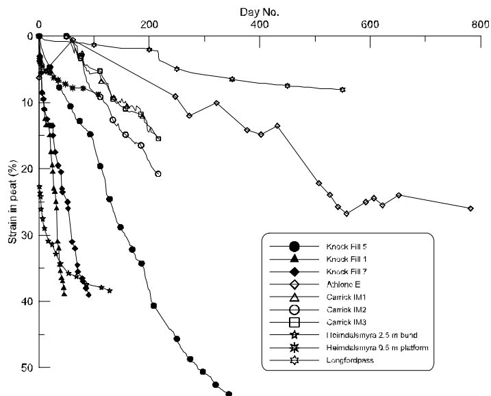
Fig 16. Strain in peat – all sites
