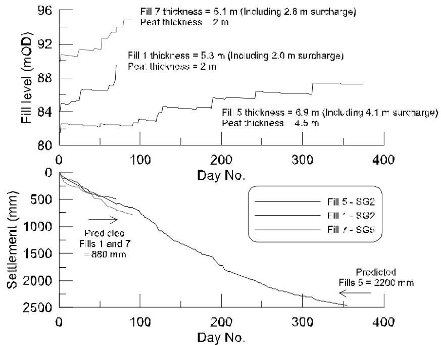
Fig 14. Knock Bypass – fill thickness and settlement data
