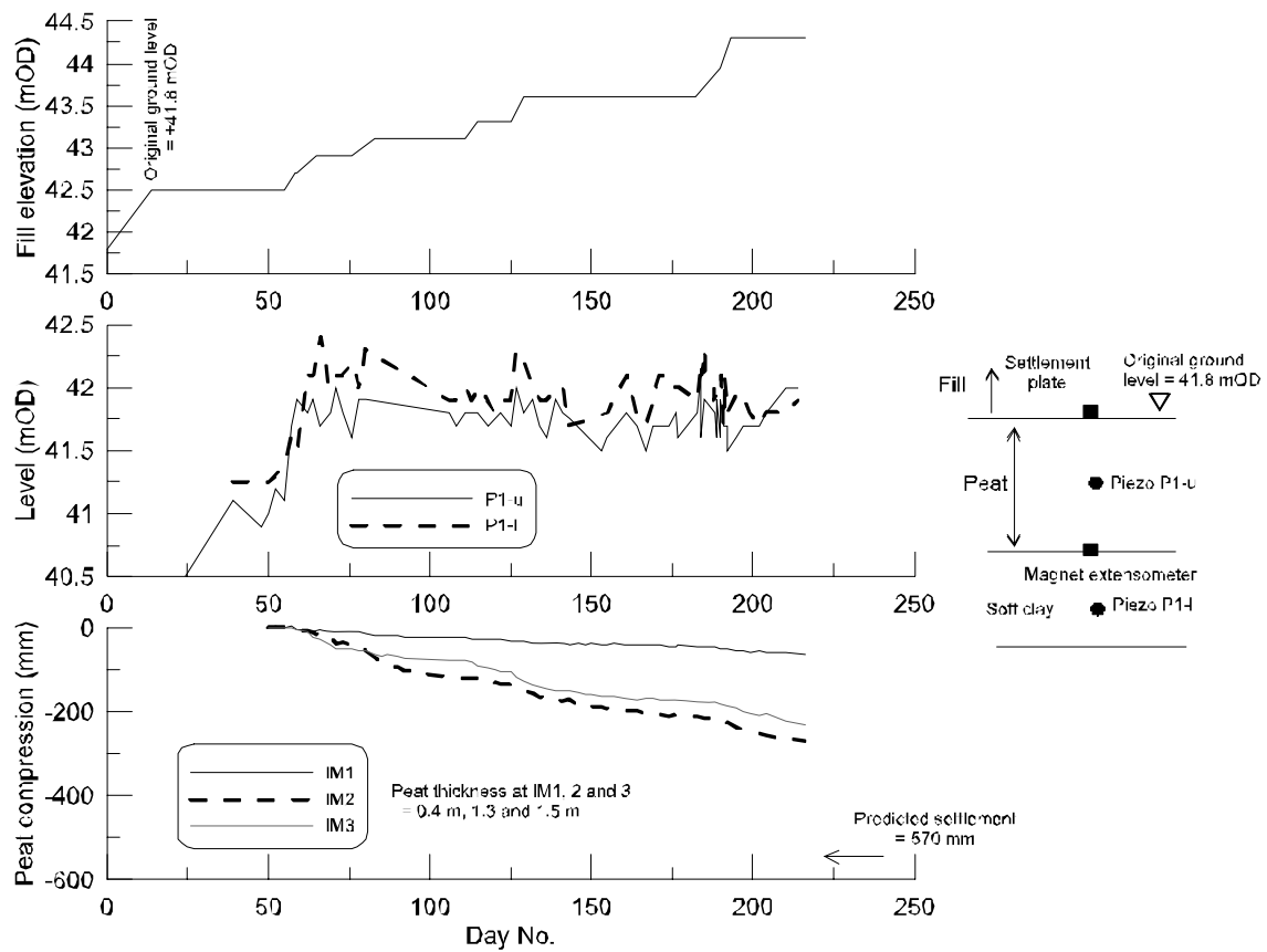
Fig 15. Carrick-on-Shannon fill thickness, porewater pressures and peat compression data
