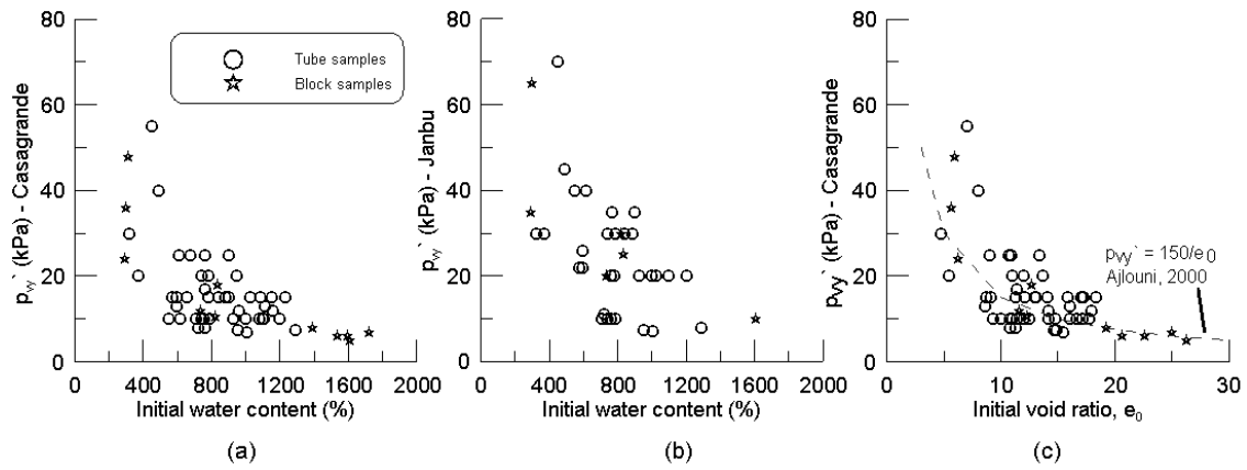
Fig. 7. Yield stress from the (a) Casagrande and (b) Janbu techniques and (c) yield stress (Casagrande) versus initial void ratio
