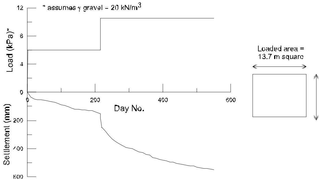
Fig 11. Longfordpass – Applied load and settlement monitoring results (Sheedy and Plant, 1968)
