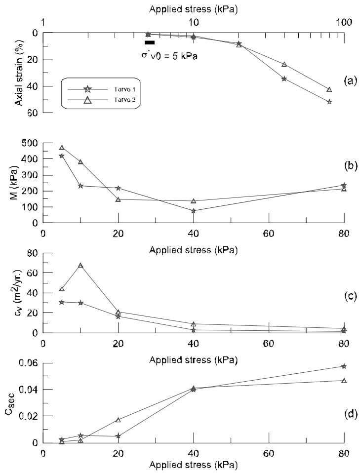
Fig. 3. Torvødometer results – Charlestown (a) \log \sigma'_v \nu \epsilon , (b) \sigma'_v \nu M , (c) \sigma'_v \nu c_v and (d) \sigma'_v \nu C_{sec} (Torvo = Torvødometer test)
