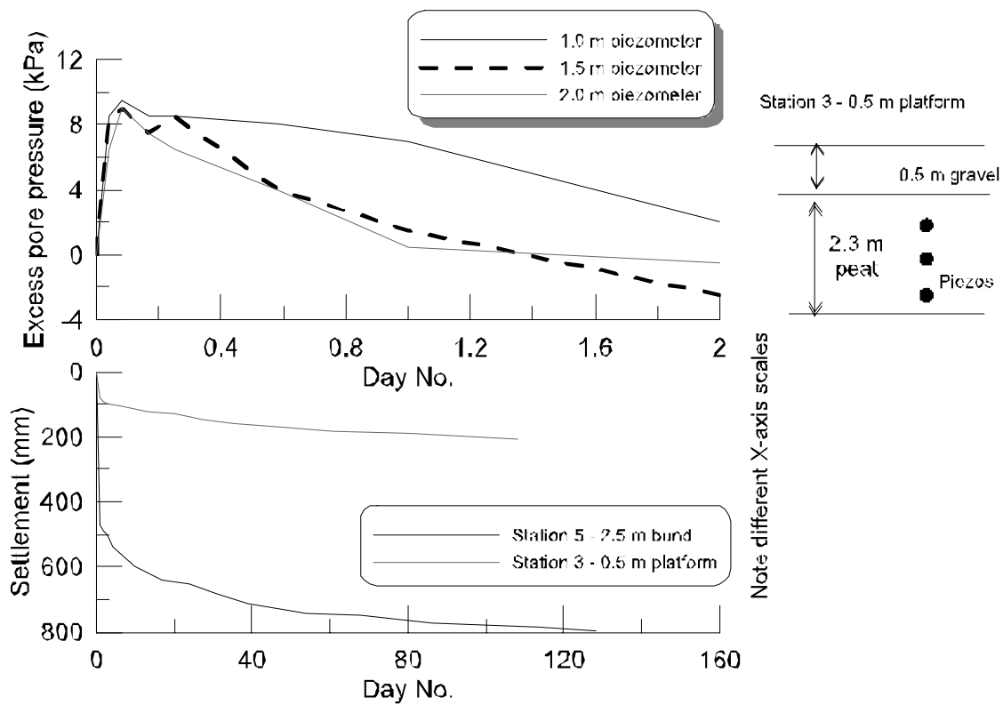
Fig 12. Heimdalsmyra – excess porewater pressure and settlement monitoring results (from Hove, 1972)
