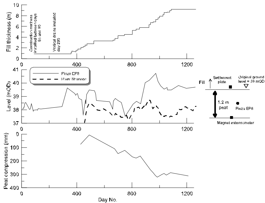
Fig 13. Athlone Bypass – fill thickness, porewater pressure and peat compression monitoring data
