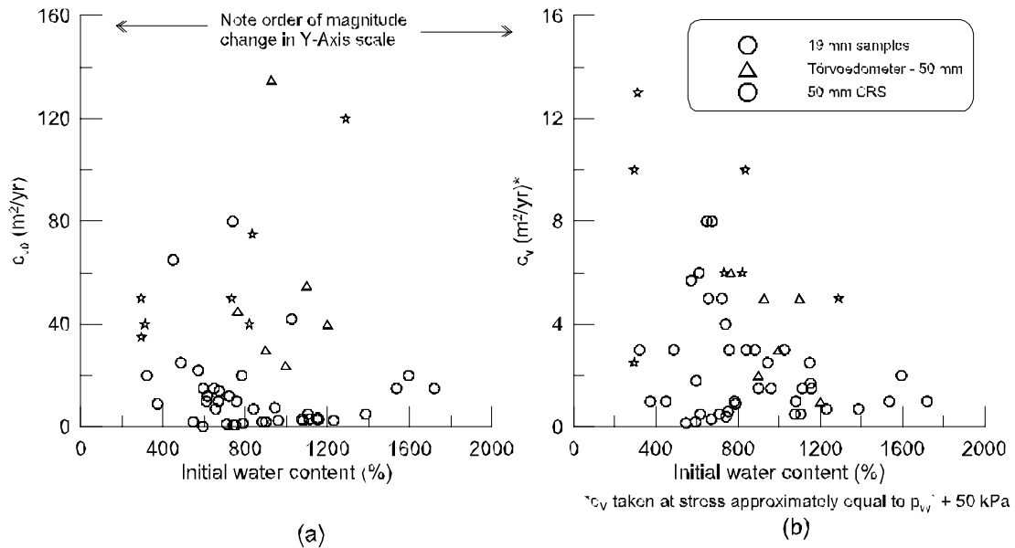
Fig 10. Coefficient of consolidation (a) at \sigma_{v0}' and (b) stress \approx p_{vy}' + 50 kPa
