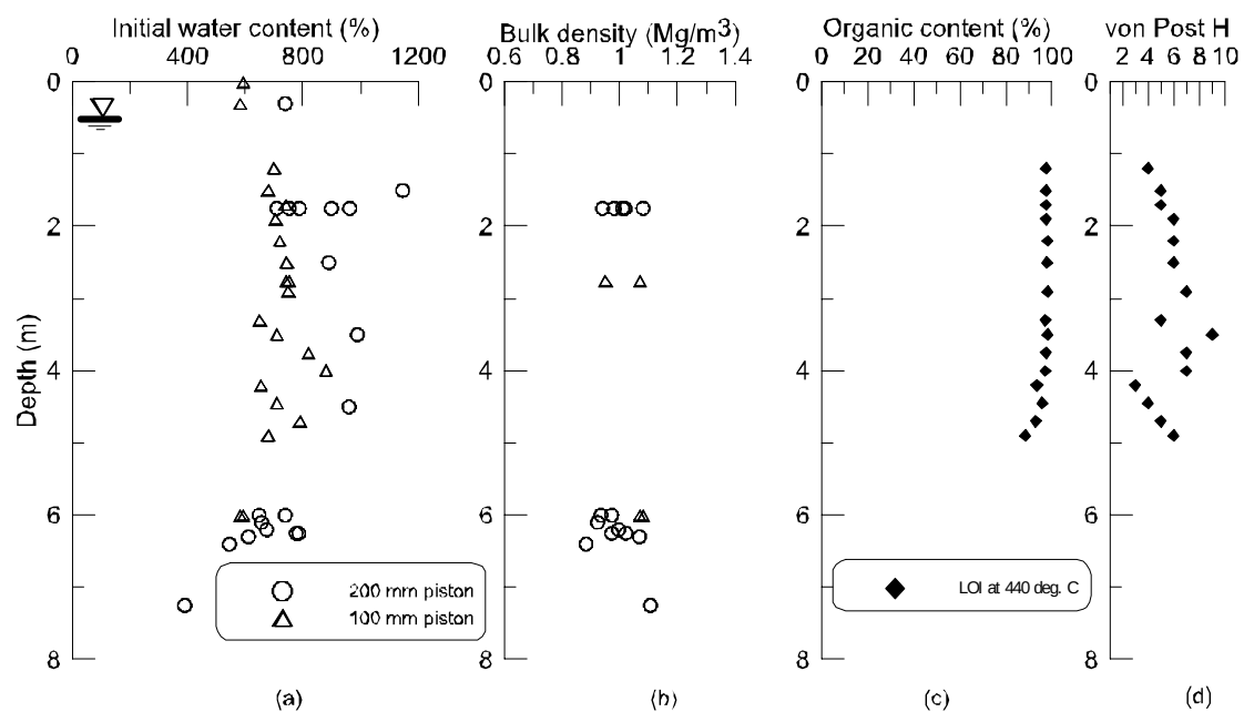
Fig. 2. Index properties – Grigg Rd., N2 site (a) initial water content, (b) bulk density, (c) organic content and (d) von Post H. Note LOI = loss on ignition.
