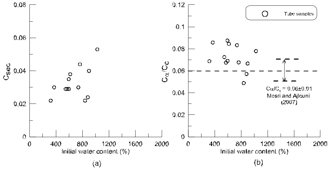
Fig. 9. Creep coefficients (a) C_{sec} and (b) C_{\alpha}/C_c (both relate to stress \approx p_{vy}' + 50 kPa)
