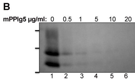
Figure 3. mPPIg5 treatment of ScN2a cells and treatment of lysates from RML and 22L infected N2a cells. A) RML infected N2a cells and 22L infected N2a#58 cells were lysed in 4% sarkosyl (in PBS pH7.4). 100 \mu g of lysate was then left untreated or treated with 2.4mg/ml of mPPIg5 dendrimers for 3 hours before analysis for protease resistant PrP Sc content by PK digestion and immunoblot. B) RML infected N2a cells were treated with increasing concentrations of mPPIg5 for 4 days before analysis by PK digest and immunoblot for PrP Sc . Apparent molecular mass based on migration of protein standards is indicated for 17, 25, and 30 kDa in both panel A and B. n = 3.
