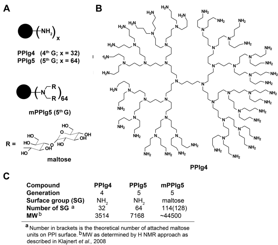
Figure 1. Schematic description of dendrimers PPIg4, PPIg5 and mPPIg5 used in this study.
