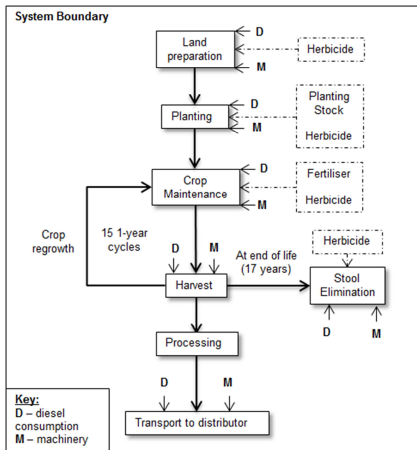
Figure 1 – System diagram
