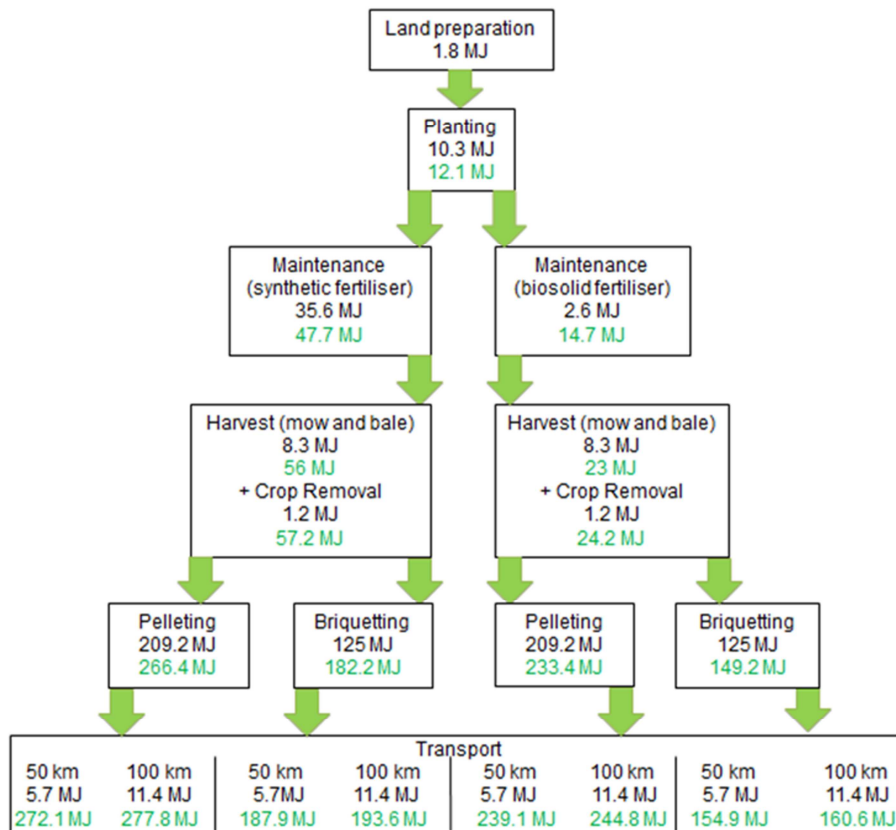
Figure 3 - Energy requirements of life cycle stages (MJ per GJ of energy produced)
