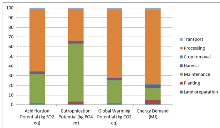
Figure 2 - Process contribution to AP, EP, GWP and CED
