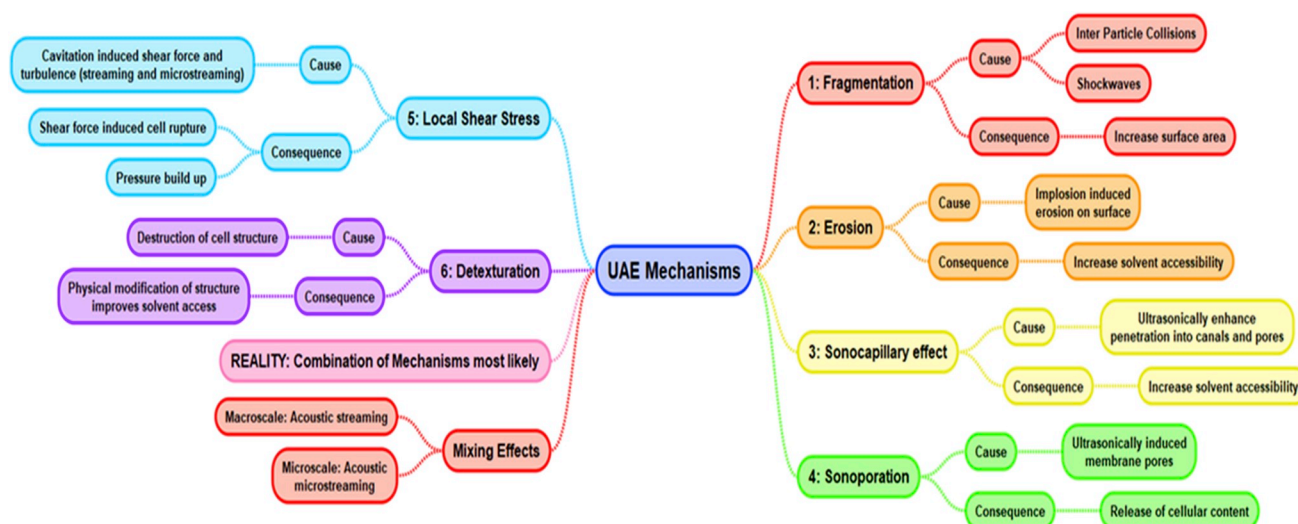
Fig. 3. Mechanisms involved in ultrasound-assisted extraction (UAE).
