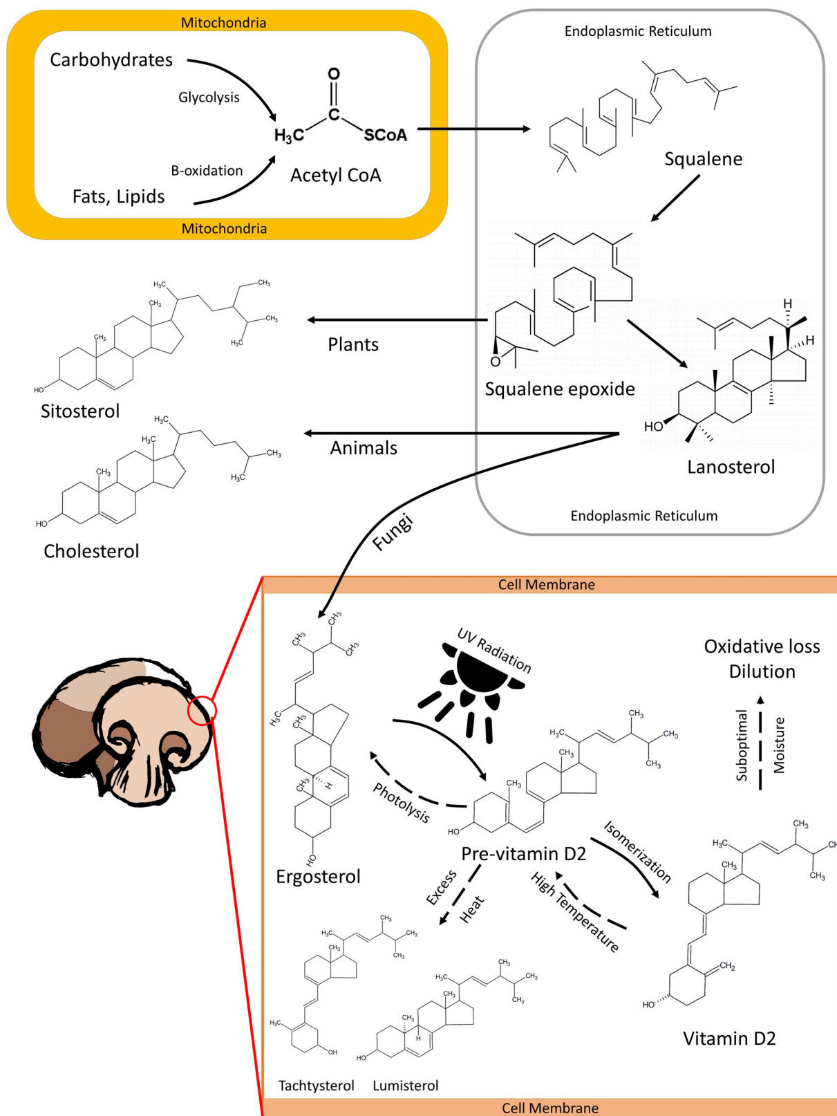
Fig. 1. Process of conversion of ergosterol into vitamin D 2 in fungal sources.
