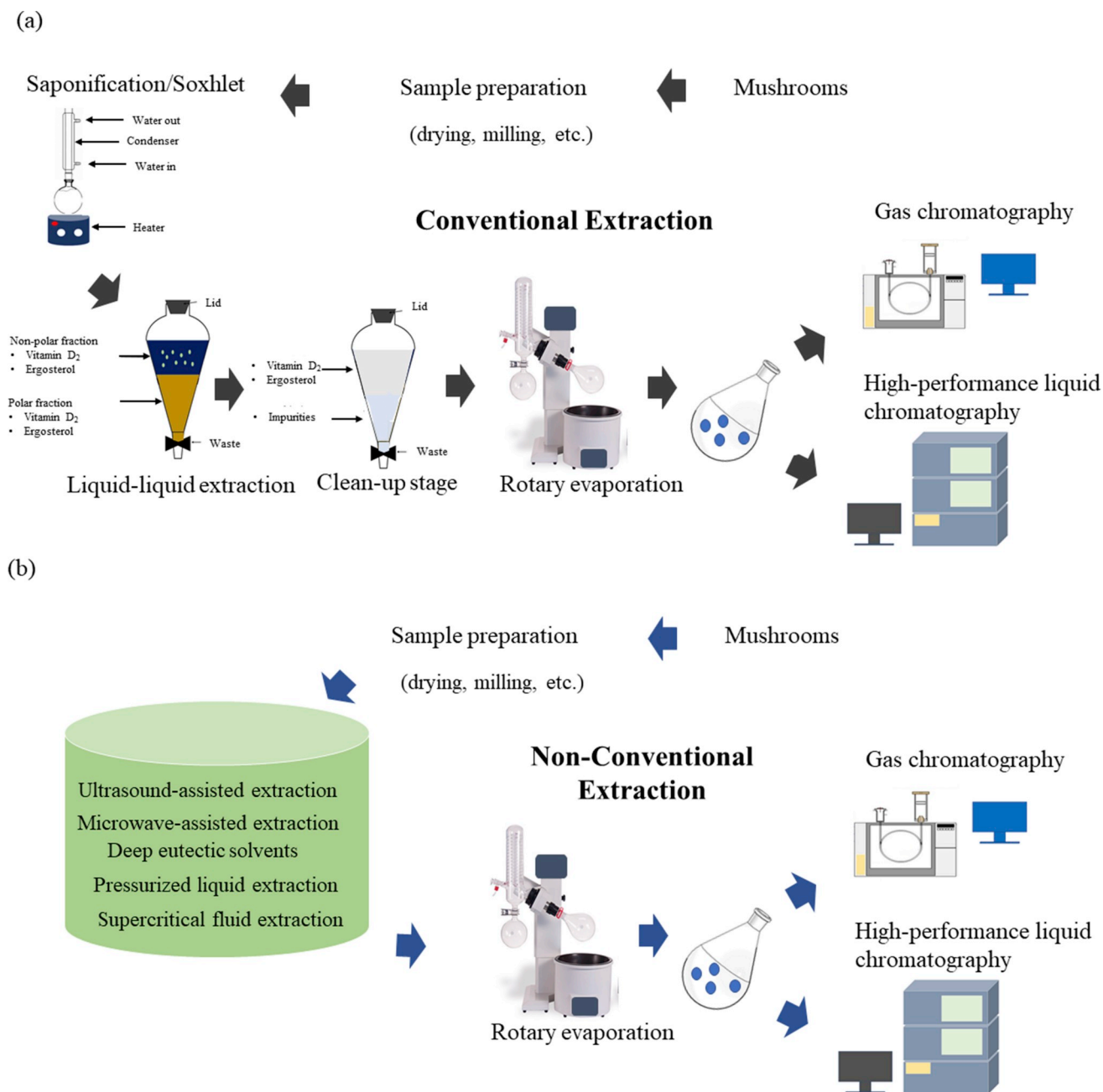
Fig. 2. Extraction and determination of ergosterol and vitamin D 2 by (a) conventional and (b) non-conventional extraction methods.
