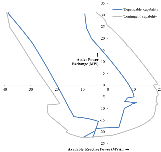
Fig. 4 Reactive power capability of the test network.
