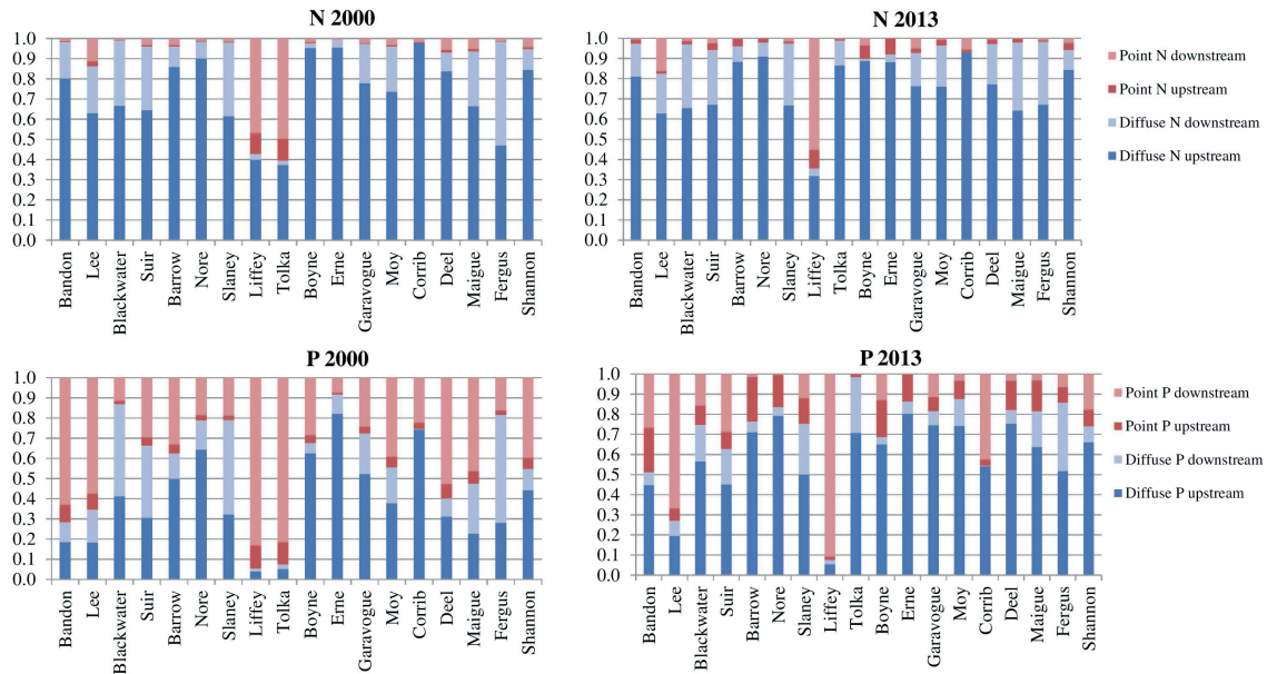
Fig. 2— Calculated nutrient load source apportionment percentage contribution for the 18 catchments studied. Point N and P relate to point sources of nutrients (wastewater treatment plants and industry) entering the estuarine system. Diffuse N and P relate to sources from agriculture, septic tanks, runoff and atmospheric deposition. Upstream sources are those above the station where riverine nutrient inputs to transitional and coastal systems are calculated (above zero salinity); downstream sources refer to those below this point (see Fig. 1).
