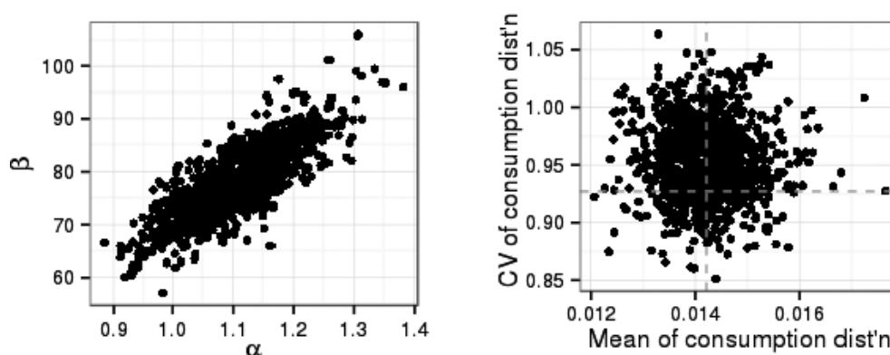
Figure B.11: Monte Carlo sample representing posterior uncertainty about parameters for the gamma distribution describing variability of consumption. The left panel shows uncertainty about the shape and rate parameters. The panel on the right shows uncertainty about the mean (kg/day) and coefficient of variation of the consumption distribution
