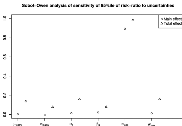
Figure B.25: Sobo–Owen analysis of sensitivity of the 95th percentile of the risk-ratio r to uncertainties about statistical parameters
