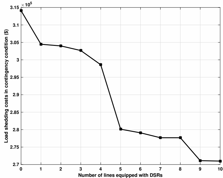
Fig. 6. Total load shedding costs ( OF_d ) in case of disaster vs number of lines equipped with DSR (Case-I)
