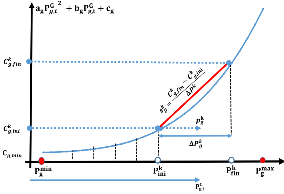
Fig. 1. Piece-wise linear fuel cost function
