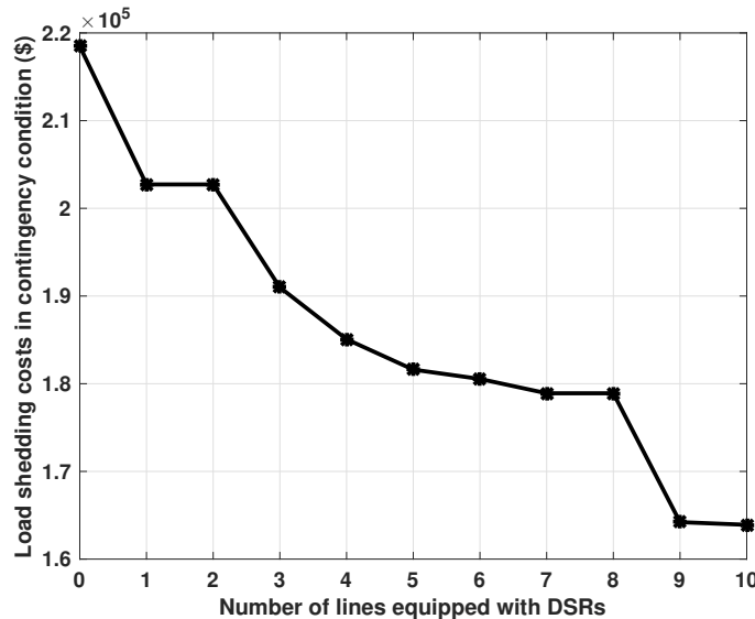
Fig. 9. Total load shedding costs ( OF_d ) in case of disaster vs number of lines equipped with DSR (Case-II)
