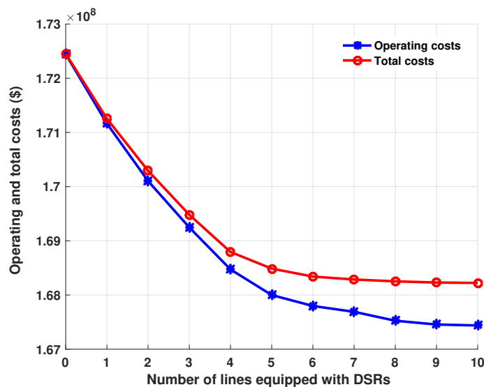
Fig. 7. Total cost and operating costs ($) vs number of lines equipped with DSR
