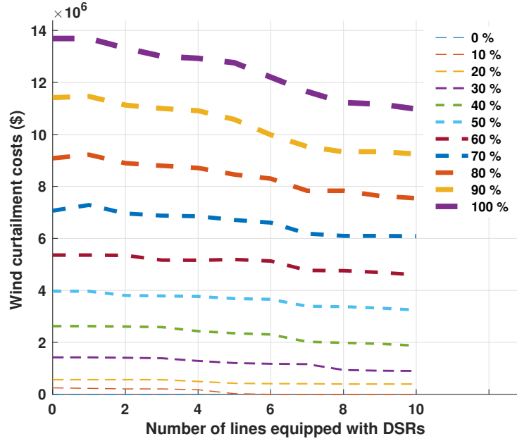
Fig. 8. Total wind curtailment cost ($) vs number of lines equipped with DSR for different percentages of increase in wind capacity
