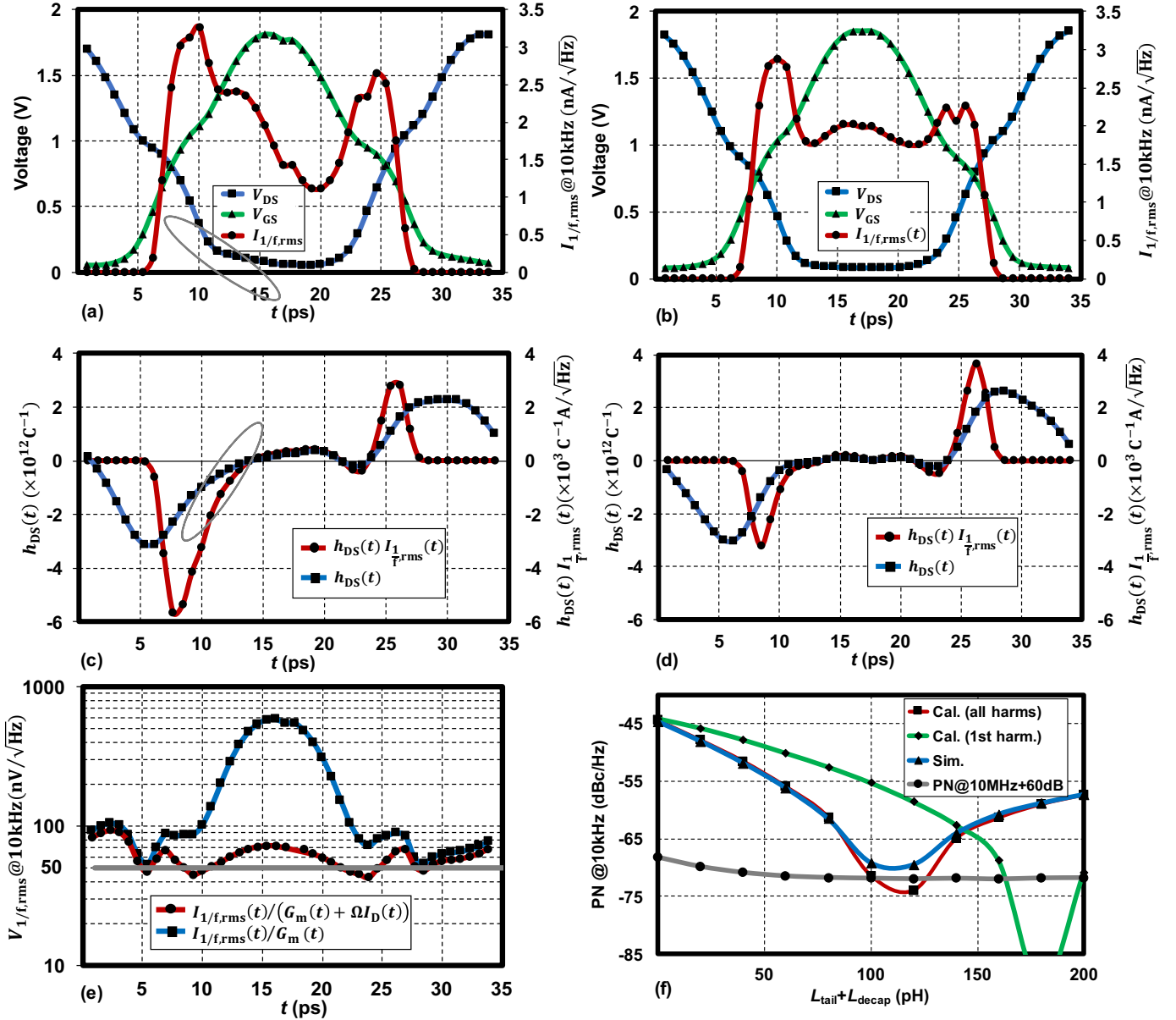
Fig. 9. Discrete waveform point of V_{\text{GS}} , V_{\text{DS}} in one period based on PSS simulations, and corresponding rms value of flicker current noise I_{1/f,rms} at 10 kHz based on DC/NOISE simulations: (a) L_{\text{tail}} + L_{\text{decap}} = 0 pH, (b) L_{\text{tail}} + L_{\text{decap}} = 120 pH (for 2nd harmonic resonance). Non-normalized ISF function h_{\text{DS}}(t) based on PXF simulations and h_{\text{DS}}(t) \times I_{1/f,rms}(t) : (c) L_{\text{tail}} + L_{\text{decap}} = 0 pH, (d) L_{\text{tail}} + L_{\text{decap}} = 120 pH. (e) Flicker noise model verification. (f) Numerical verification of PN @ 10kHz.
