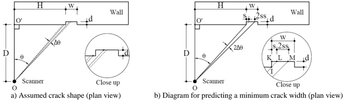
Figure 2. Schematic diagram of a wall crack and laser scanner
