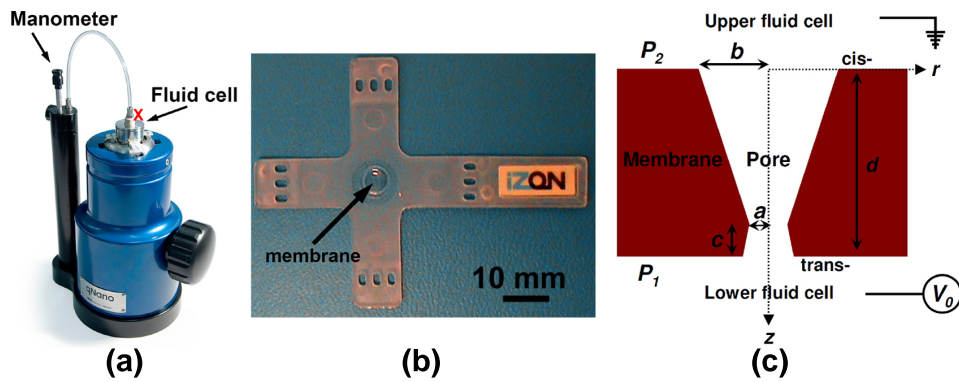
FIG. 1: The setup for tunable pore experiments. Figure 1(a) shows the qNano apparatus with the specimen, fluid cell and manometer unit in place. To apply a magnetic field, a small bar magnet was placed on top of the fluid cell, adjacent to the manometer attachment (at the red “x”). Figure 1(b) shows the elastomeric specimen, which enables actuation of a pore within the thin central membrane. A schematic cross-section of a pore is shown in Fig. 1(c). A pore constriction of radius a is located a distance c from the lower membrane surface, and the opening at the upper surface has radius b . The membrane thickness is d , the transmembrane potential is V_0 , the downwards pressure head is P_2 - P_1 , and the r and z co-ordinates of a cylindrical polar co-ordinate system are indicated.
