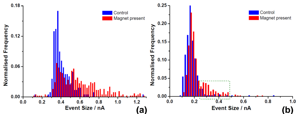
FIG. 6: Magnitude histograms for experiments N4 (Fig. 6(a)) and N6 (Fig. 6(b)) using data collected by the automated detection process. The dashed green box in Fig. 6(b) highlights a significant variation between the ‘control’ and ‘magnet present’ modes.
