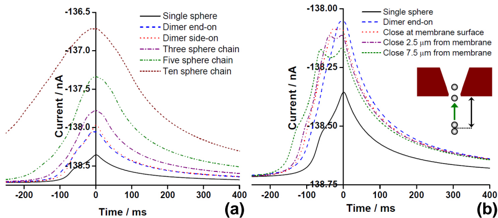
FIG. 5: Simulated resistive pulses, calibrated using parameters for the control mode in experiment N4. Figure 5(a) compares simulations of particle ‘chains’ of various lengths translocating lengthwise, and for a dimer passing through the pore side-on. Figure 5(b) compares results for a single sphere and an end-on dimer with various cases in which two particles are transported independently of each other. Simulations are set up so that sphere surfaces are ‘close’ (less than 50 nm apart) at some distance from the membrane surface. This distance is indicated by the black double arrow in the inset schematic section of the pore. Particles become more separated at the pore constriction, where the flow velocity gradient is maximised.
