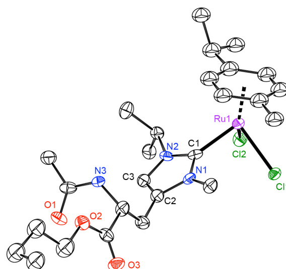
Fig. 1 ORTEP plot of complex 6a (50% probability, hydrogen atoms omitted for clarity). Selected bond lengths (Å) and angles (°): Ru1–C1 2.067(10), Ru1–Cl1 2.407(3), Ru1–Cl2 2.430(3), Ru1–C centroid 1.691(5), C1–Ru1–Cl1 88.4(3), C1–Ru1–Cl2 89.1(3), Cl1–Ru1–Cl2 84.0(1).
