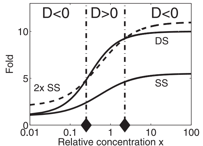
Figure 9. Illustration of a re-entrant dose response predicted by the thermostatical model for a double-binding-site promoter. The solid line ‘DS’ was computed from Eq. (25) and represents the fold change of the transcriptional activity of a double binding site promoter for a given relative transcription factor concentrations x . The solid line labeled ‘SS’ represents the transcriptional activity of a corresponding single binding site promoter (as computed from Eq. (82) given in Text S1). The dashed line represents two times the activity calculated for the single binding site promoter. Diamonds indicate the critical transcription factor concentrations x_c calculated from Eq. (91) in Text S1. As expected, these critical values correspond to the critical values that can be obtained directly from the intersections of the ‘2x SS’ and ‘DS’ graphs. Parameters: q_R = 0.1 , \Omega_{Rx} = 10 , \Omega_{xx} = 1 , and \Omega_{Rxx} = 1 . doi:10.1371/journal.pone.0034439.g009
