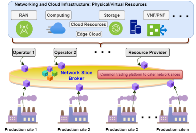
Fig. 1: Role of network slice broker to enable FaaS.
