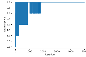
(b) Convergence performance of WoLF-PHC algorithm: Fog node/slice optimal demand of one resource
