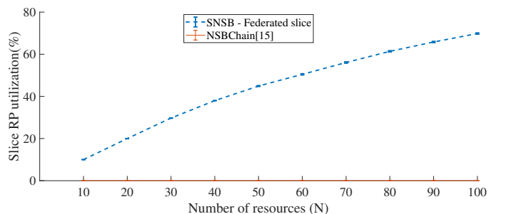
Fig. 9: Resource provider utilization - NSBChain vs SNSB
