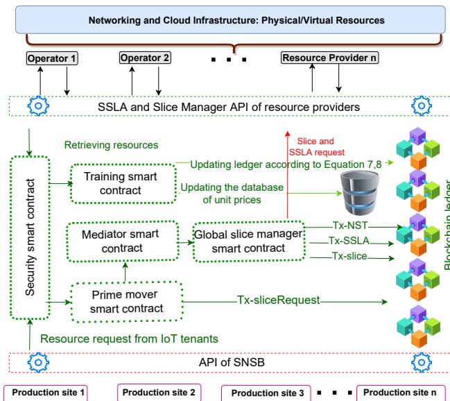
Fig. 4: Smart contract interaction
