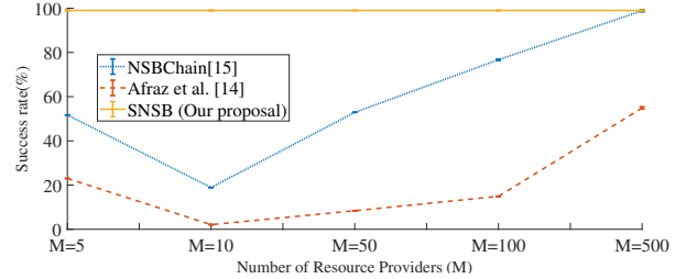
(a) Success rate on scaling up the number of resource providers
