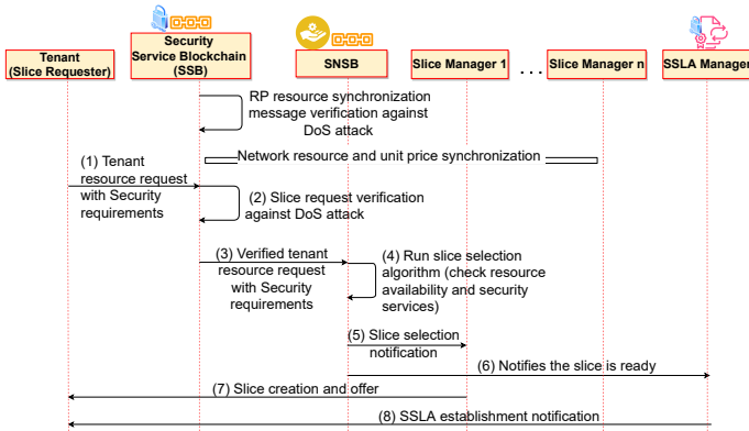
Fig. 3: The workflow of brokering architecture
