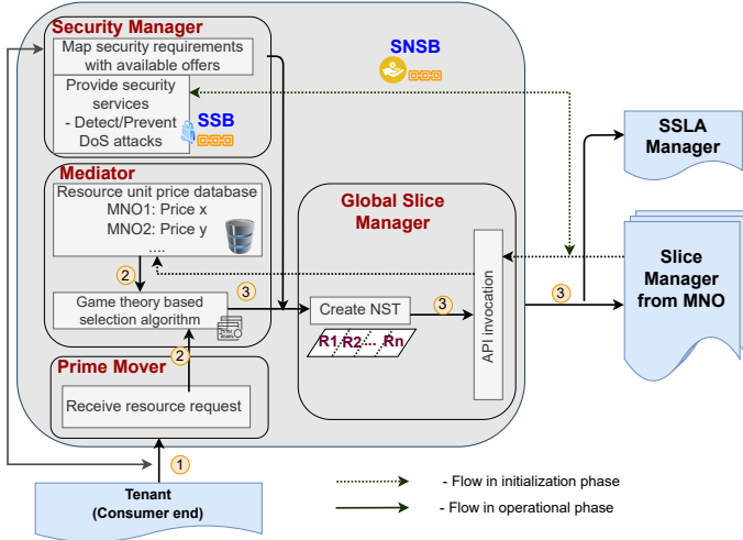
Fig. 2: The proposed architecture of SNSB solution
