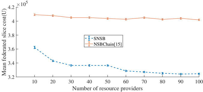
Fig. 10: Offer price comparison - NSBChain vs SNSB
