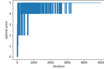
(a) Convergence performance of WoLF-PHC algorithm: Resource provider optimal price of one resource
