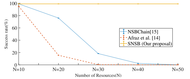
(b) Success rate on scaling up the number of resources
