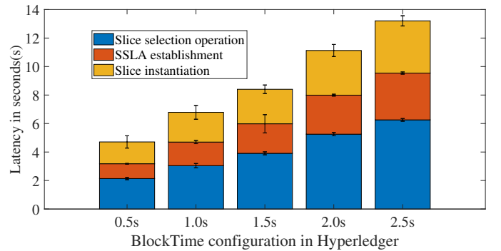
Fig. 8: End-to-end slice creation latency
