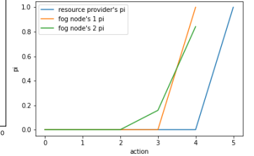
(c) Agent's \pi values in the state when other agents play optimal action
