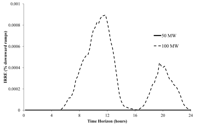
Fig. 7. Downward IRRE test system results with 50 MW and 100 MW of wind generation capacity
