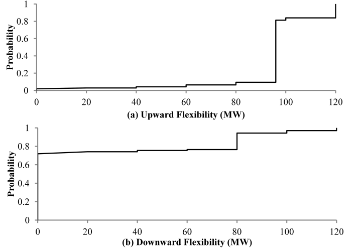
Fig. 4. \text{AFD}_{15min.}(X) in (a) upward and (b) downward directions
