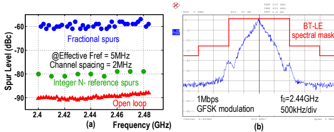
Fig. 7. (a) ADPLL fractional, reference and open-loop spurs; (b) Bluetooth GFSK modulation spectrum.
