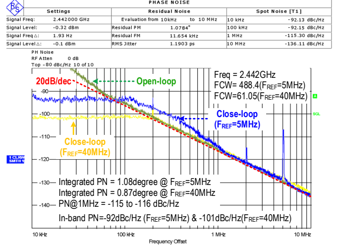
Fig. 6. Transmitter phase noise in open-loop and different close-loop configurations.
