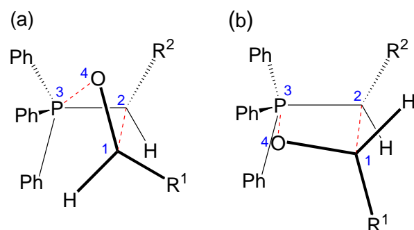
Fig. 9. Cycloaddition TSs leading to OPA in Wittig reactions of alkylidetriphenylphosphoranes: (a) kinetically favoured cis -selective cycloaddition TS showing a positive angle of pucker, with R^2 in a pseudo-axial site and R^1 in a pseudo-equatorial site; (b) lowest energy trans -selective TS. R^1 is the large carbonyl substituent, and R^2 is the large ylide \alpha -substituent.
