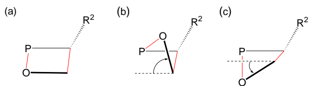
Fig. 8. (a) Planar TS with pucker angle of 0^\circ , (b) TS with positive pucker angle, (c) TS with negative pucker angle.
