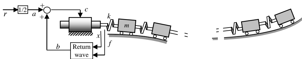
Fig.5: Quasi rectilinear system experiencing changing external forces from gravity requiring a modified WBC
