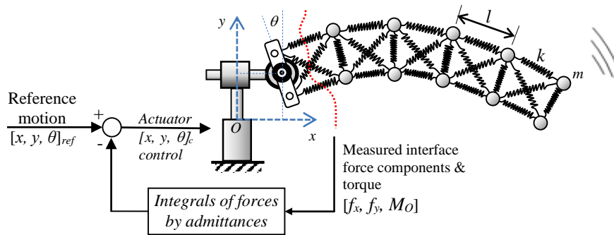
Fig.3: Planar mass-spring array controlled by actuator which translates and rotates.
