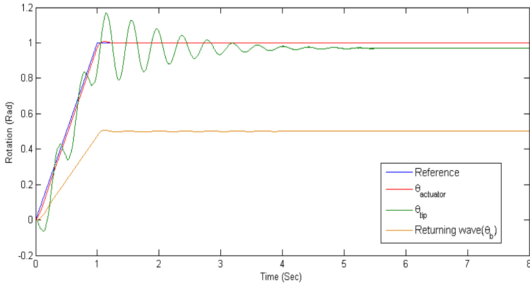
Fig.7: A rotational maneuver under gravity using WBC and the control system of Fig.4.
