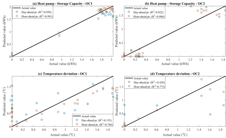
Figure 14: Actual (white-box) and predicted values (BCNN), hourly up-flex DR actions: (a) heat pump storage capacity — OC1, (b) heat pump storage capacity — OC2, (c) temperature deviation — OC1.
