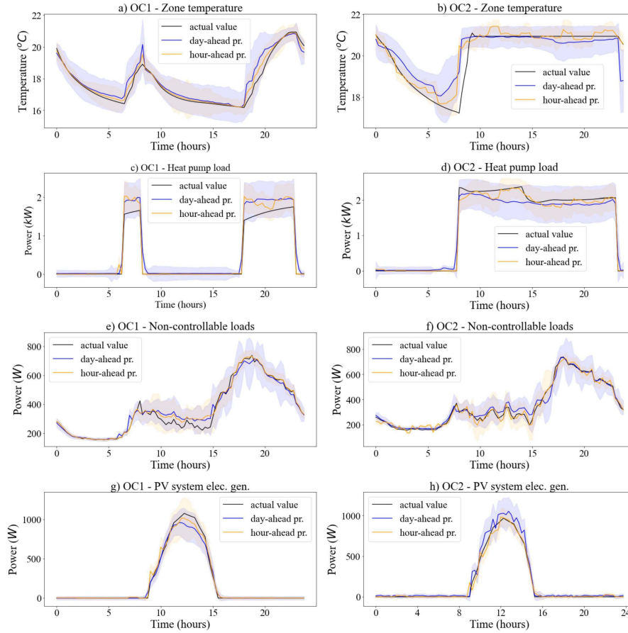
Figure 7: Predicted (BCNN), 95% prediction intervals, and actual (white-box) values: Zone temperature: (a) OC1, (b) OC2, Heat pump load: (c) OC1, (d) OC2, Non-controllable loads: (e) OC1, (f) OC2, PV electricity generation: (g) OC1, (h) OC2.
