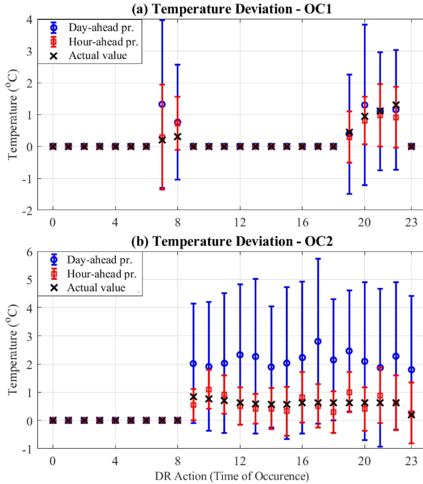
Figure 16: Hourly uncertainty map of the temperature deviations (hourly down-flex DR actions): (a) OC1, (b) OC2.
