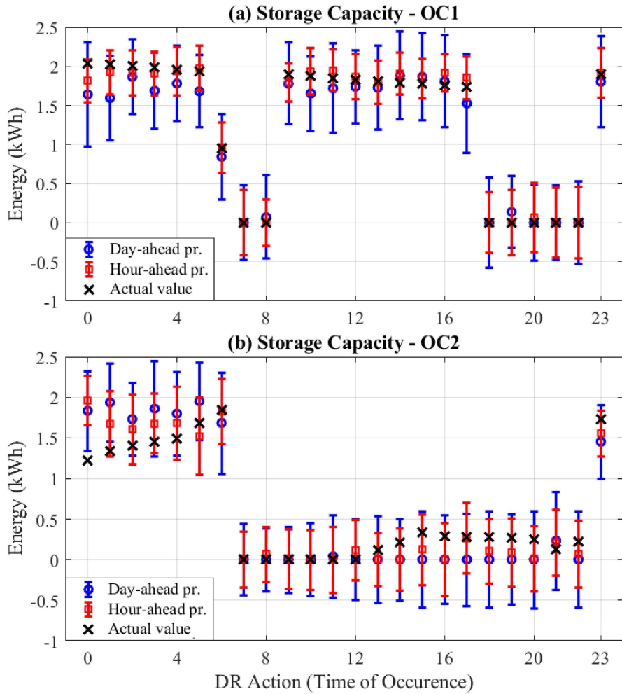
Figure 18: Hourly uncertainty map of the heat pump storage capacity (hourly up-flex DR actions): (a) OC1, (b) OC2.
