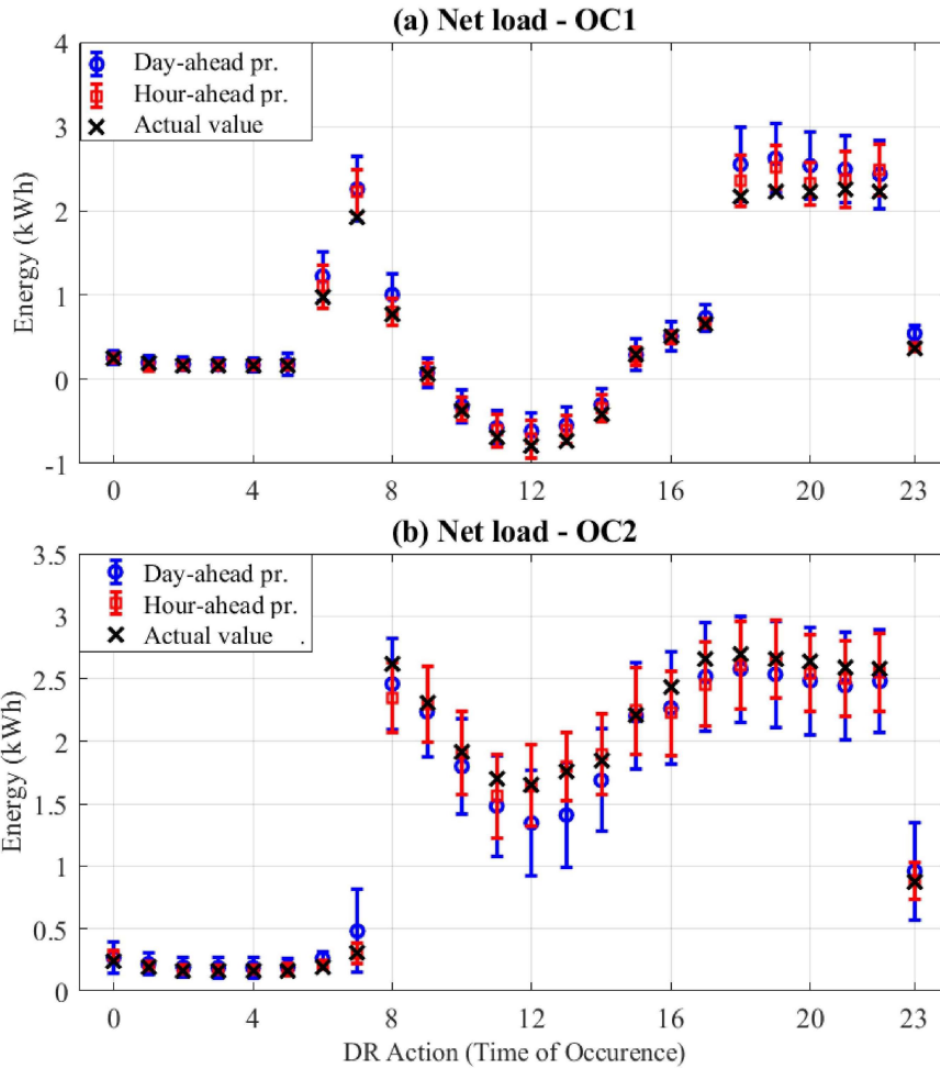
Figure 17: Hourly uncertainty map of the battery storage capacity (hourly down-flex DR actions): (a) OC1, (b) OC2.
