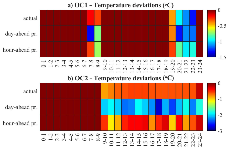
Figure 9: BCNN predicted temperature deviations (hourly down-flex DR actions): (a) OC1, (b) OC2.
