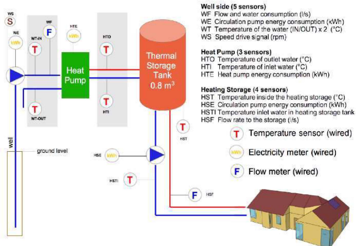
Figure 3: Heat system design and sensor metering [66].
