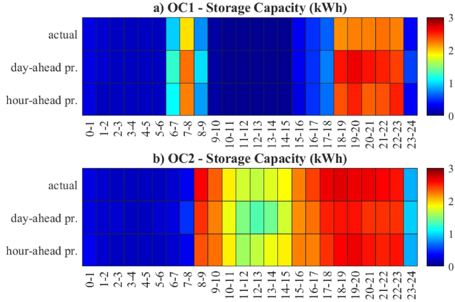
Figure 10: BCNN predicted battery storage capacity ( C_{DF} ) (hourly down-flex DR actions): (a) OC1, (b) OC2.
