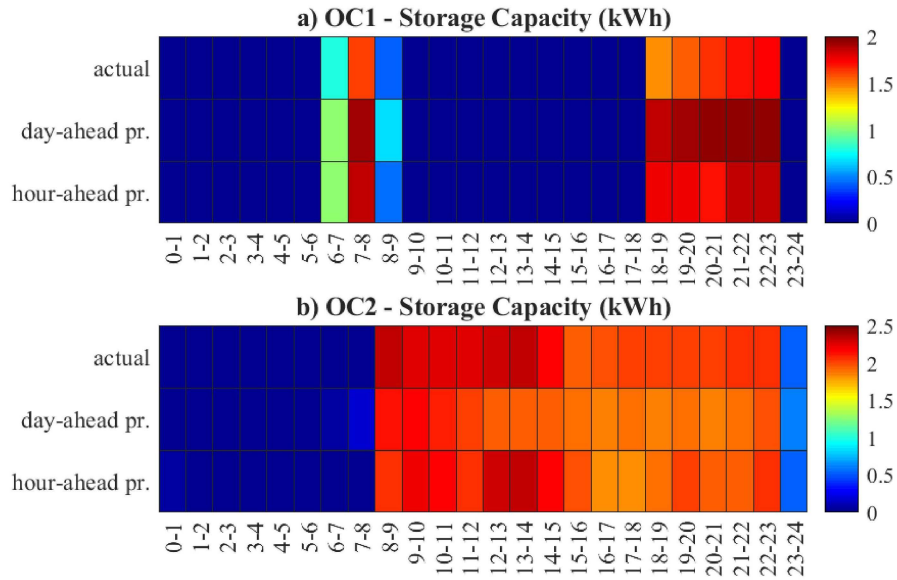
Figure 8: BCNN predicted heat pump storage capacity ( C_{DF} ) (hourly down-flex DR actions): (a) OC1, (b) OC2.
