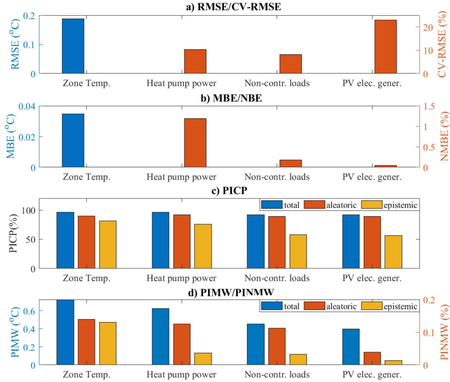
Figure 5: (a) RMSE/CV-RMSE, (b) MBE/NMBE, (c) PICP, (d) PIMW/PINMW for each target variable (zone temperature, heat pump load, non-controllable loads, PV system electricity generation), hour-ahead prediction models.
