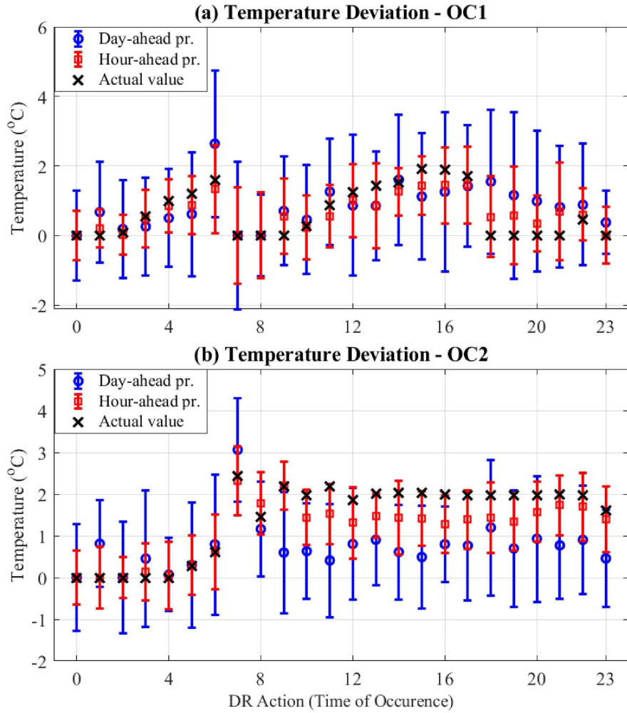
Figure 19: Hourly uncertainty map of the temperature deviations (hourly up-flex DR actions): (a) OC1, (b) OC2.
