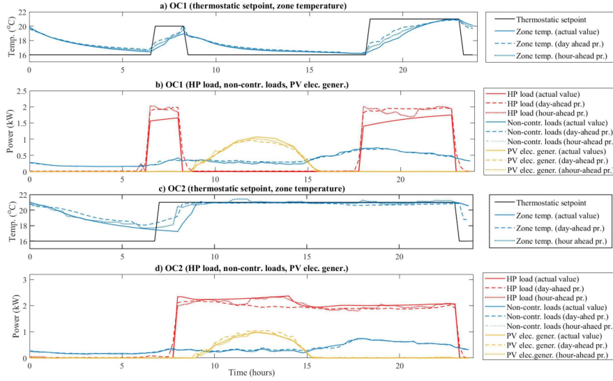
Figure 6: Predicted (day-ahead (dashed), hour-ahead (dotted)) and actual (continuous) values: (a) Thermostatic setpoint and zone temperature, OC1, (b) heat pump load (red), non-controllable loads (blue), PV electricity generation (yellow), OC1, (c) Thermostatic setpoint and zone temperature, OC2, (d) heat pump load (red), non-controllable loads (blue), PV electricity generation (yellow), OC2.
