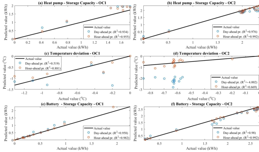
Figure 11: Actual (white-box) and predicted values (BCNN), hourly down-flex DR actions: (a) heat pump storage capacity — OC1, (b) heat pump storage capacity — OC2, (c) temperature deviation — OC1, (d) temperature deviation — OC2, (e) battery storage capacity — OC1, (f) battery storage capacity — OC2.
