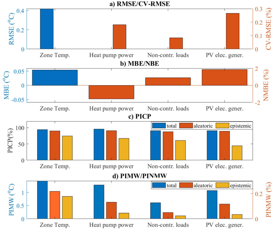
Figure 4: (a) RMSE/CV-RMSE, (b) MBE/NMBE, (c) PICP, (d) PIMW/PINMW for each target variable (zone temperature, heat pump load, non-controllable loads, PV system electricity generation), day-ahead prediction models.
