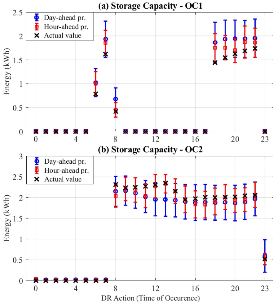
Figure 15: Hourly uncertainty map of the heat pump storage capacity (hourly down-flex DR actions): (a) OC1, (b) OC2.
