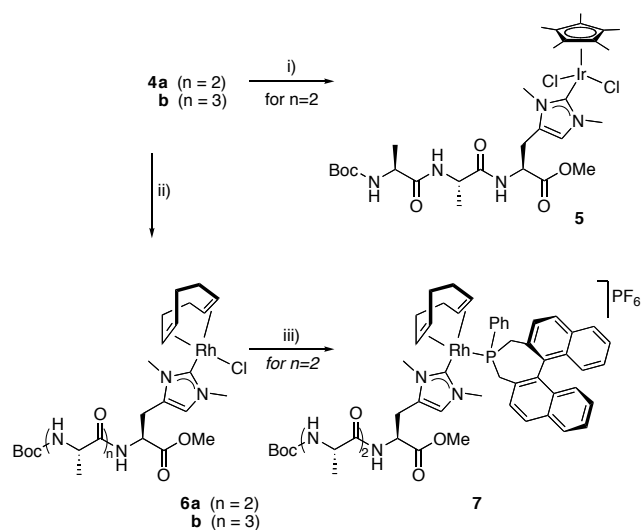
Scheme 2 Synthesis of alanine-containing histidylidene iridium 5 and rhodium 6–7 complexes. Reagents and conditions: i) Ag 2 O, [Ir(Cp*)Cl 2 ] 2 , CH 2 Cl 2 , rt; ii) Ag 2 O, [Rh(cod)Cl] 2 , CH 2 Cl 2 , rt; iii) ( S )-Ph-binepine, KPF 6 , CH 2 Cl 2 /H 2 O, rt.
