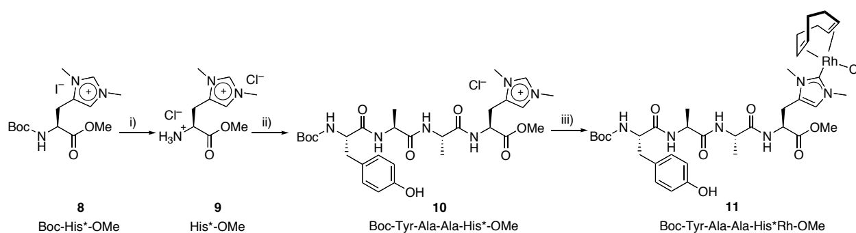
Scheme 3 Synthesis of the peptide-embedded histidylidene-rhodium complex 11 containing a tyrosine residue. Reagents and conditions: i) HCl/1,4-dioxane, rt, then ion-exchange resin; ii) Boc-Tyr-Ala-Ala-OH, HATU, DIEA, THF, rt, then ion-exchange resin; iii) [NET 3 Me]I, Ag 2 O, [Rh(cod)Cl] 2 , CH 2 Cl 2 , rt.
