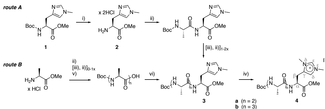
Scheme 1 Synthesis of the histidinium tripeptide 4a and tetrapeptide 4b . Reagents and conditions: i) HCl/MeOH, reflux; ii) Boc-Ala-OH, HATU, DIEA, THF, rt; iii) HCl/1,4-dioxane, rt; iv) MeI, MeCN, 40 °C; v) LiOH, THF/MeOH/H 2 O, rt, then HCl aq.; vi) 2 , HATU, DIEA, THF, rt.
