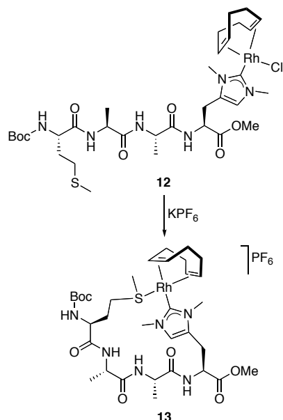
Scheme 4 Caption methionine analogues 12 and 13 featuring a monodentate and chelating bidentate bonding mode of the histidylidene, respectively
