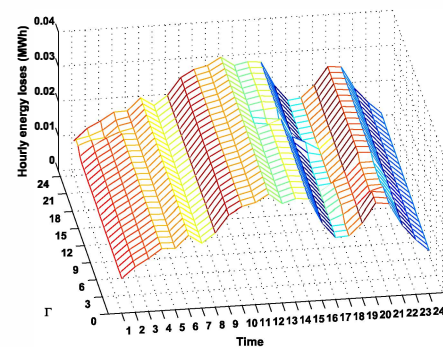
Fig. 9. The hourly energy losses vs \Gamma in controlled case
