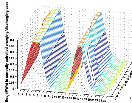
Fig. 8. The state of charge vs \Gamma in centrally controlled case
