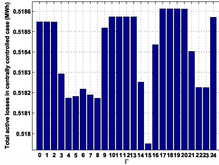
Fig. 10. The total energy losses vs \Gamma in controlled case
