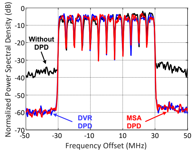
Fig. 4. Signal Spectrum with and without DPD.
