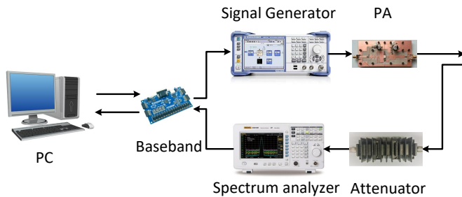
Fig. 3. DPD test bench.
