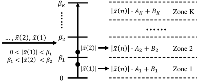
Fig. 1. Magnitude-selective affine function.
