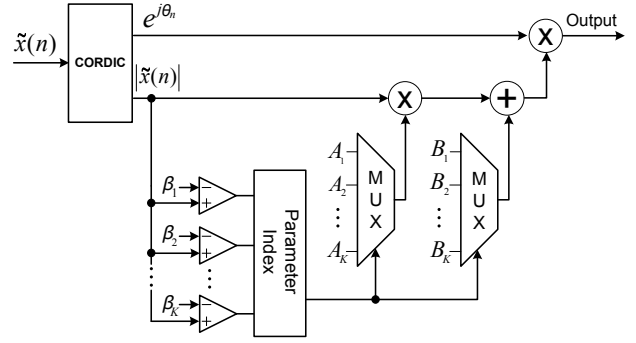
Fig. 2. Hardware implementation illustration.
