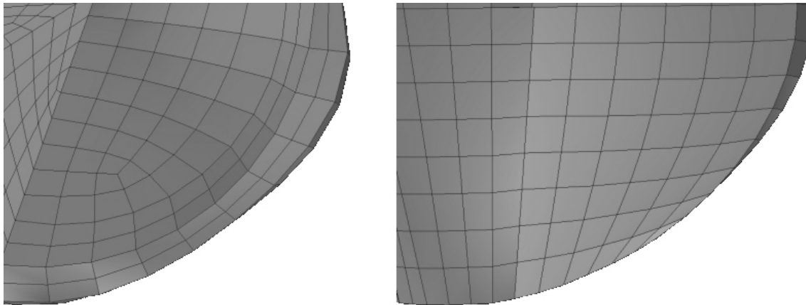
Figure 7: Comparison of element quality in projection mesh model (left) with baseline model (right). Note the large internal angles in the outer elements of the baseline model as compared to those in the projection mesh model.
