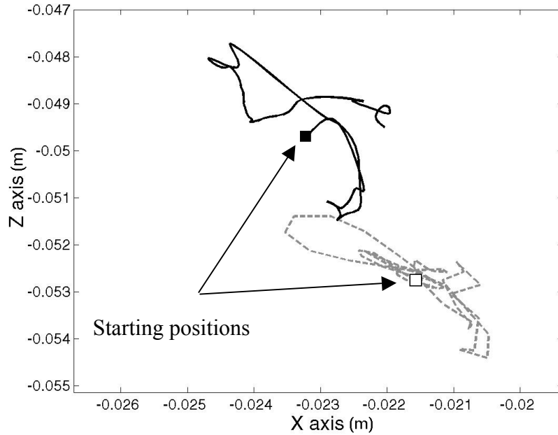
Figure 13: Close up on path taken by NDT 6 in experiment (black solid line) and path taken by the closest equivalent node in the simulation (grey dashed line). The solid black box indicates the starting position for the experimental data while the open black box is the initial position of the adjacent node.
