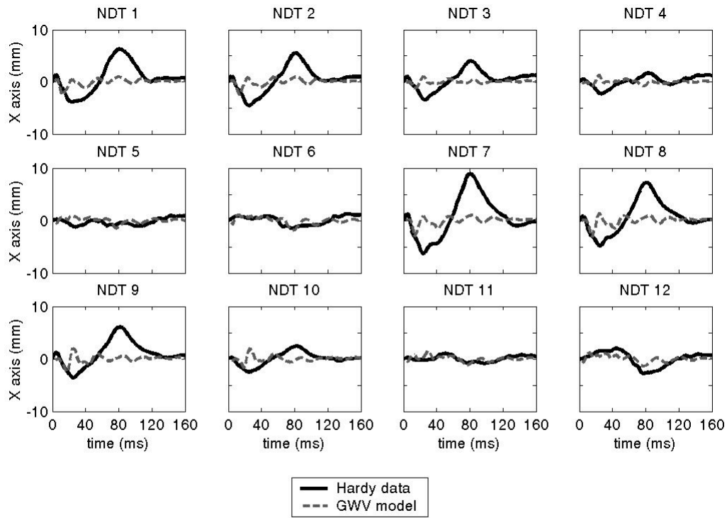
Figure 15: Comparison of the simulated relative displacements against the data of Hardy et. al. [3] for the GWV model. Displacements here are in the local X direction. The accuracy of the more inferior markers (1-4, 7-10) is poorer than those of the superior markers (5, 6, 11 and 12), where more simulated brain motion takes place.
