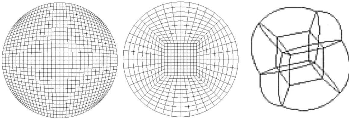
Figure 5: The swept mesh method (a) is simple to implement but will not be numerically well-conditioned if only quadrilateral elements are used. The projection mesh method involves two meshing steps but combines good element quality throughout the resulting mesh with the complete use of quadrilateral (b) and hexahedral elements (c). Images courtesy of the TrueGrid homepage [38].
