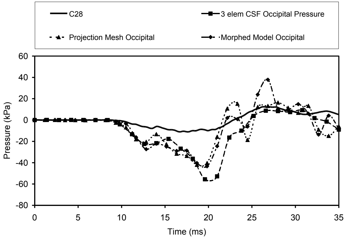
Figure 10: Comparison of remaining 3 models' pressure response versus the Trosseille experimental data.
