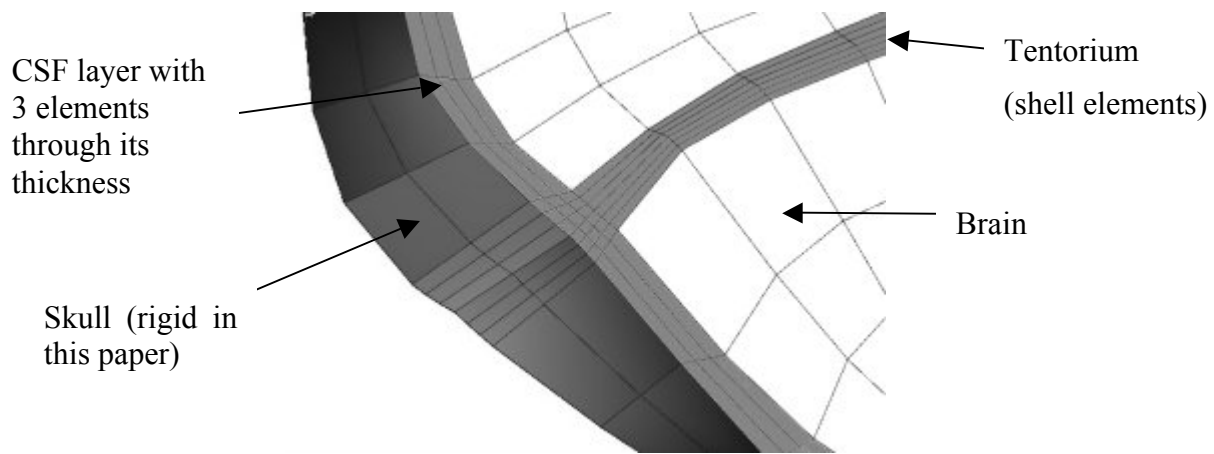
Figure 4: Detail of CSF layer when three elements were placed through the thickness rather than one. The size of the resulting elements between the skull and the intracranial membranes required the use of adaptive meshing.
