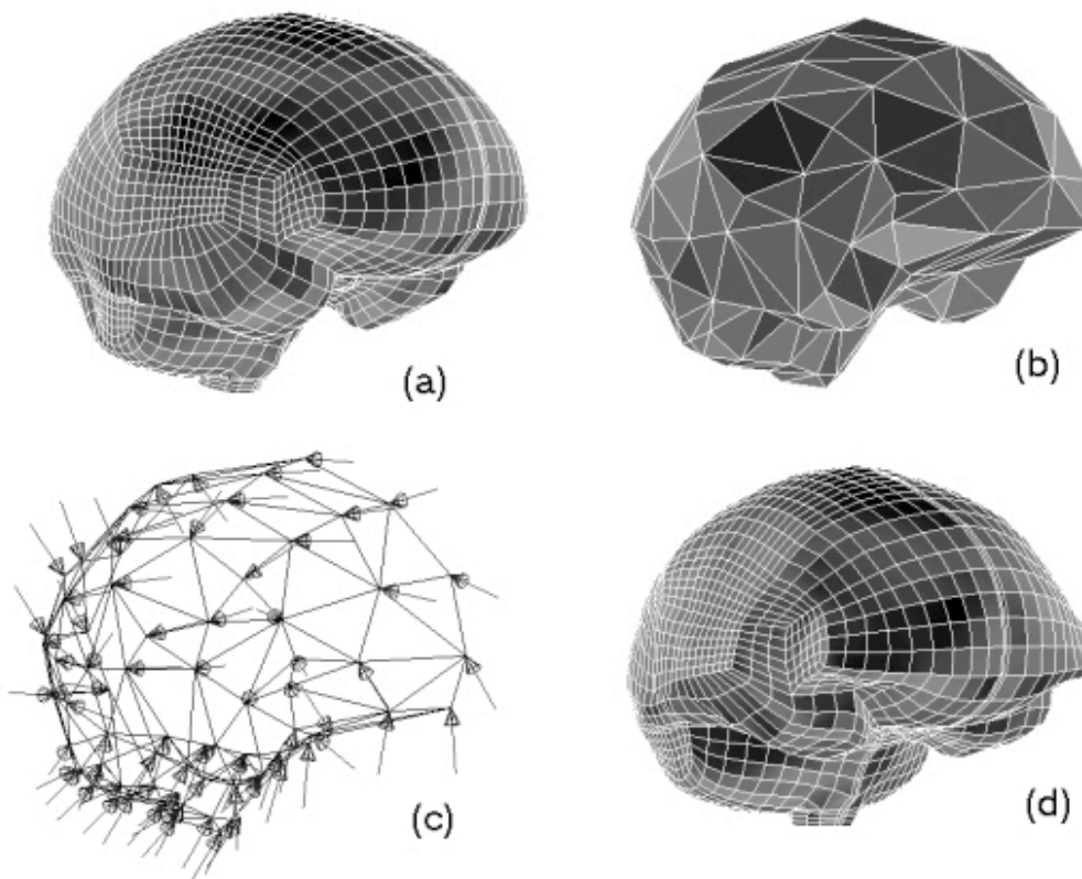
Figure 8: Steps used to make the morphed model. A coarse grid (b) was constructed on the original model (a). A Discrete field of displacement vectors were then applied to every node of this coarse grid (half of which are visible in (c)), and this field was converted into a continuous field in order to create (d). The morphed model is of Van Lierde and Vander Sloten [42] while the original model is of the visible male [32].
