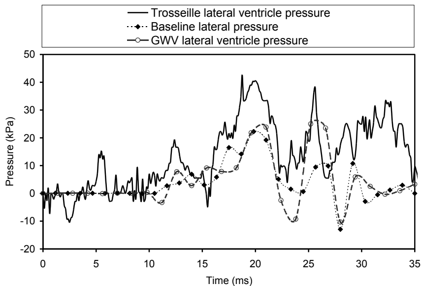
Figure 11: Comparison of experimental and simulated pressures at the lateral ventricle for the baseline and the GWV model. Pressure is measured at the same element for both models.
