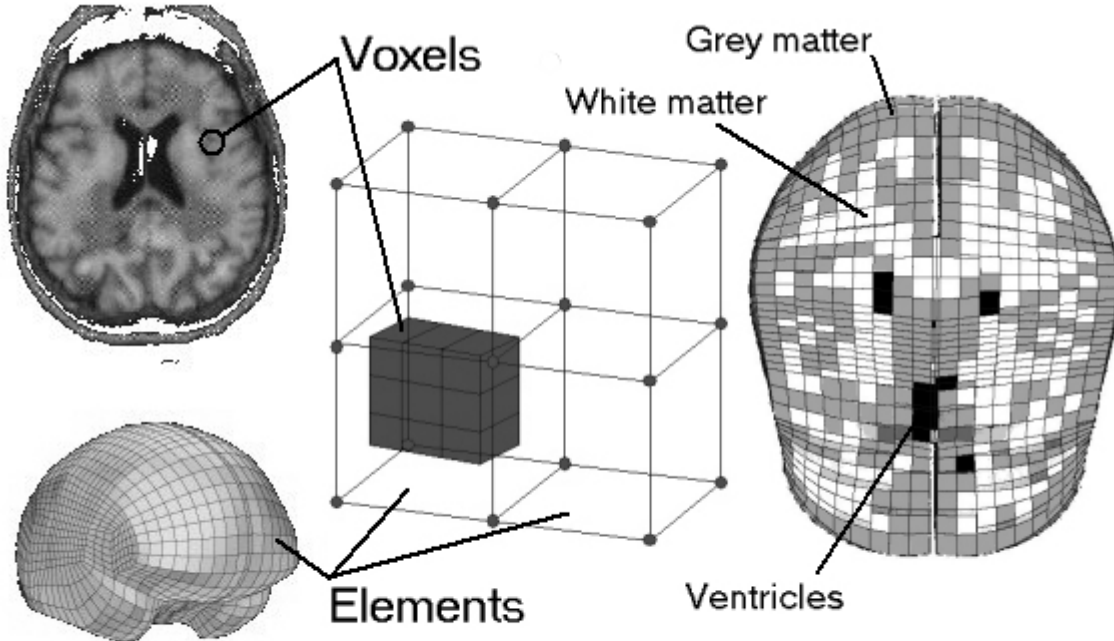
Figure 2: The basis upon which the purpose-written MATLAB program works involves two steps to assign specific material properties to the elements of the cerebrum. The MRI voxels and finite elements within the FE model are registered to occupy the same space. Each element identifies which voxels are contained within its six faces. By an appropriate choice of threshold values of voxel intensities, the element is assigned the constitutive properties for grey, white or ventricular matter, although the MATLAB program can assign intermediate properties to each element uniquely.
