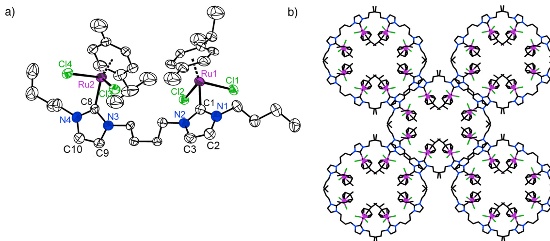
Figure 3. a) ORTEP representation of 2d (30% probability ellipsoids; H atoms and co-crystallized Et 2 O molecule omitted for clarity) and b) packing diagram showing the channel-type ordering of the molecules.
