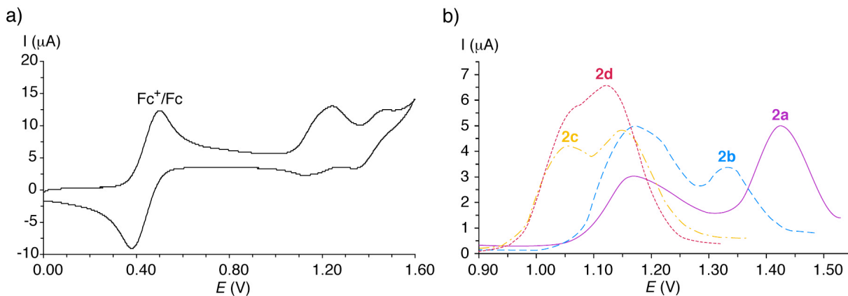
Figure 4. a) Cyclic voltammogram of complex 2a ( \text{Fc}^+/\text{Fc} as internal reference) and b) differential pulse voltammograms of 2a–d .
