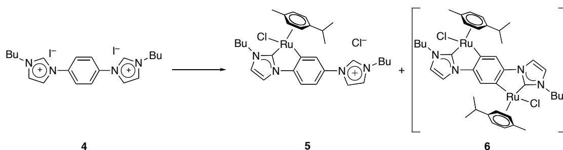
Scheme 2. Synthesis of phenylene-bridged Ru II –NHC complexes. Reagents and conditions: Ag 2 O, CH 2 Cl 2 , 40 °C, 16 h, then [RuCl 2 (cymene)] 2 , CH 2 Cl 2 , 40 °C, 16 h.
