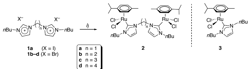
Scheme 1. Synthesis of bimetallic ruthenium(II) carbene complexes 2 and the corresponding monometallic model compound 3 ; reagents and conditions: i) \text{Ag}_2\text{O} , MeCN, +40 °C, 16 h, then [\text{RuCl}_2(\text{cymene})]_2 , \text{CH}_2\text{Cl}_2 , -196 °C to RT or RT, 16 h.
