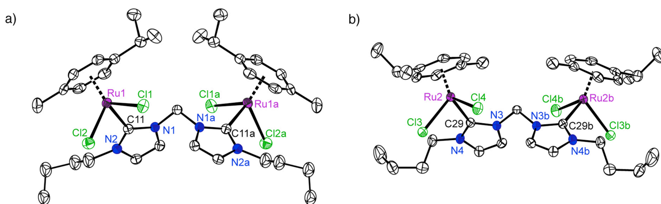
Figure 2. ORTEP representation of the two independent molecules in the unit cell of complex 2a (50% probability ellipsoids, H atoms omitted for clarity; only one of the two disordered positions of the \text{CH}_2\text{CH}_3 moiety of the n Bu group is shown in a).
