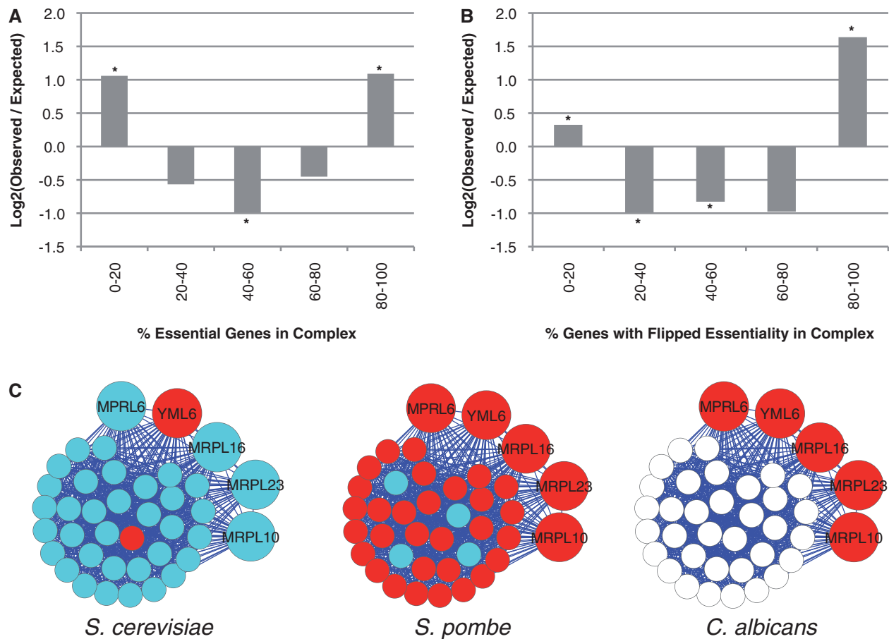
Fig. 4. — Schizosaccharomyces pombe complexes exhibit modular essentiality, and complexes flip essentiality between the two yeast species. (A) Experimentally characterized S. pombe complexes exhibit modular essentiality. The observed distribution of essential genes is compared with that expected at random, as in figure 1C (See Materials and Methods). (B) Protein complexes flip essentiality between S. pombe and S. cerevisiae . The observed distribution of “flipped” genes is compared with that expected at random, as in figure 1C. Only genes present in a single copy in both species are used for this analysis. The complex definitions are the same as those used for S. cerevisiae , as they have greater coverage than S. pombe . (C) The mitochondrial ribosomal large subunit. This complex is essential in S. pombe and Candida albicans but nonessential in S. cerevisiae . White circles correspond to genes whose essentiality status has yet to be experimentally determined. Genes whose orthologs have unknown essentiality status in C. albicans are unlabeled and shown as smaller circles.
