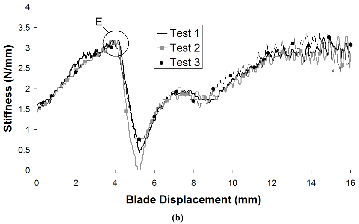
Figure 7 Indentation cutting with blunt SM blades; (a) Load-deflection curves, (b) corresponding stiffness-deflection curves
