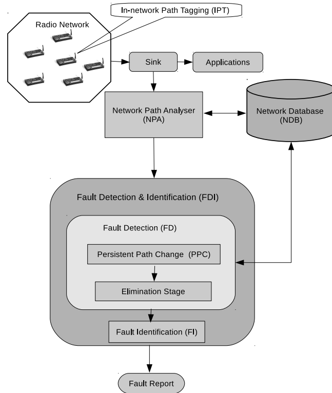
Fig. 2. SBFDF framework.
