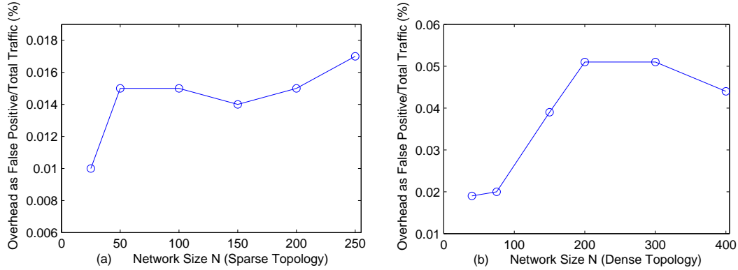
Fig. 10. Message overhead due to False Positive w.r.t. total traffic of the network (a) Sparse (b) Dense
