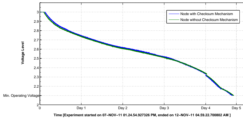
Fig. 7. RN internal voltage level variation with time (min. operating voltage = 2.1V).
