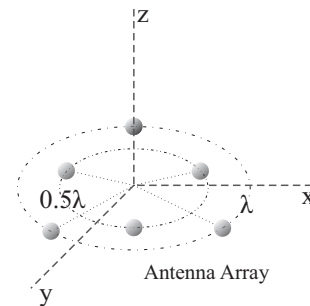
Fig. 2. ANTENNA ARRAY WITH 6 SENSORS
