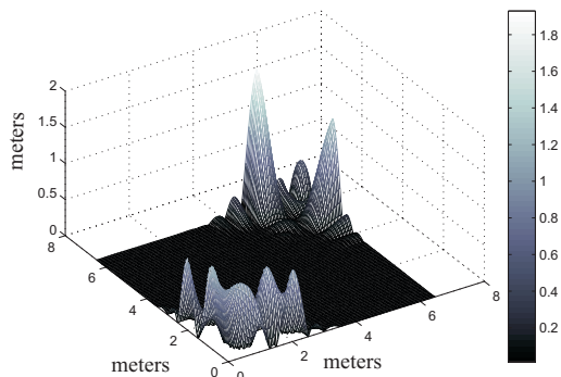
Fig. 7. ERROR SURFACE FOR A 6X6X4 METERS ROOM WITH DIRECTIONAL TRANSDUCERS
