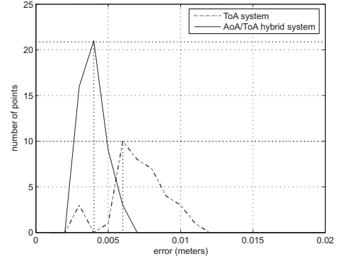
Fig. 5. ERROR ESTIMATION INTO A 10dB SNR ROOM, OMNI-DIRECTIONAL TRANSDUCERS
