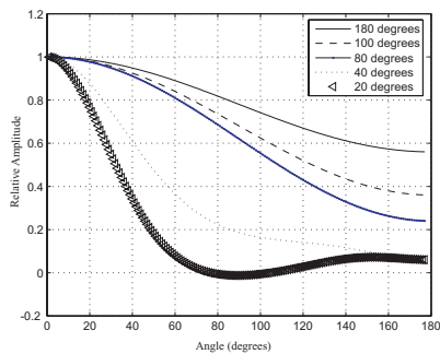
Fig. 6. TRANSDUCERS DIRECTIONAL RESPONSE
