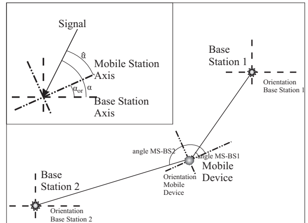
Fig. 1. ORIENTATION PROBLEM AND SOLUTION WITH 2 BASE STATIONS
