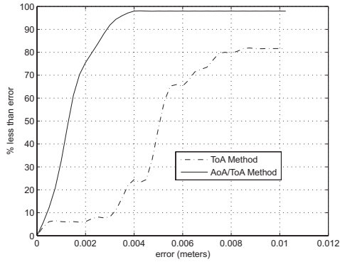
Fig. 4. LOCATION ESTIMATES WITH ERROR OF LESS THAN X METERS AT 10 DB SNR, OMNI-DIRECTIONAL TRANSDUCERS
