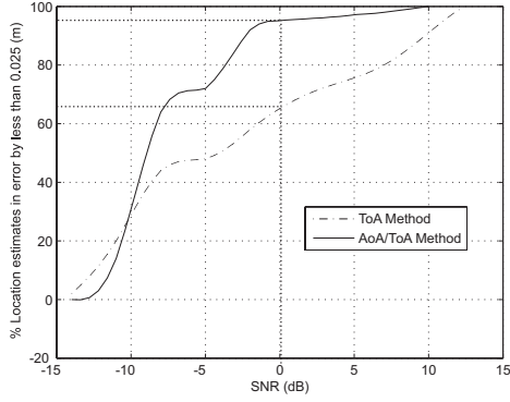
Fig. 3. LOCATION ESTIMATES IN ERROR BY LESS THAN 0.025 METERS, OMNI-DIRECTIONAL TRANSDUCERS
