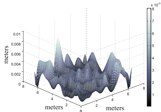
Fig. 8. ERROR SURFACE FOR A 6X6X4 METERS ROOM WITH OMNI-DIRECTIONAL TRANSDUCERS
