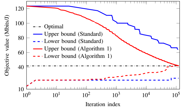
Fig. 1. Convergence of the optimal algorithms over a random channel realization. We take b_{\text{max}} = 4 .
