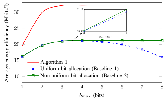
Fig. 2. Average EE performance versus the maximum number of quantization bits b_{\text{max}} .
