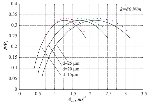
FIG. 2: Normalised power \Pi as a function of the acceleration amplitude A_{ext,opt} belonging to the optimal line. The spring constant is k = 80 and the three different lines corresponds to different rest gaps d = 15 , d = 20 and d = 25 \mu\text{m} . The circles show the normalised power calculated from the numerical simulations for comparison with theoretical results.
