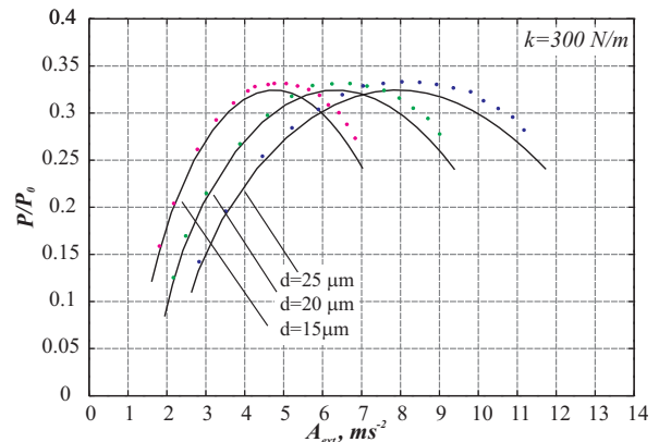
FIG. 3: Normalised power \Pi as a function of the acceleration amplitude A_{ext,opt} belonging to the optimal line. The spring constant is k = 300 and the three different lines corresponds to different rest gaps d = 15 , d = 20 and d = 25 \mu\text{m} .
