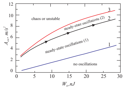
FIG. 1: Plane of parameter (W_0, A_{ext}) where the different areas correspond to different regimes displayed by the system. Line 1 is shows the onset (necessary condition) of steady-state oscillations, line 2 is the doubling bifurcation and line 3 is transition to irregular motion and chaos.
