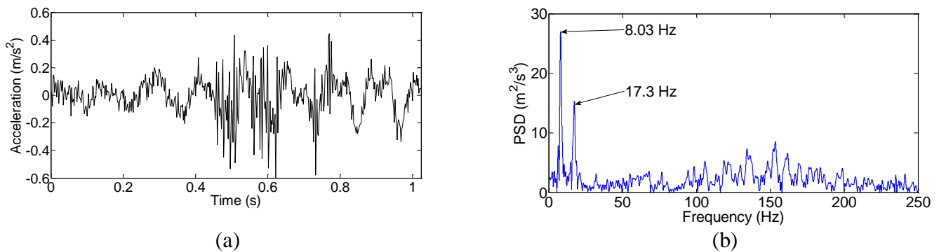
Fig. 25. Mid-span acceleration response (at 3 m from bridge centreline in lane 1) corrupted with 5% noise versus time of a bridge with an elasto-plastic region at 9 m: (a) time domain; (b) frequency domain
