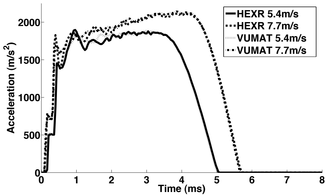
Figure 8: Comparison of acceleration time traces between HAX and VUMAT for 50\text{kg/m}^3 foam with a Poisson's ratio of 0.2.
