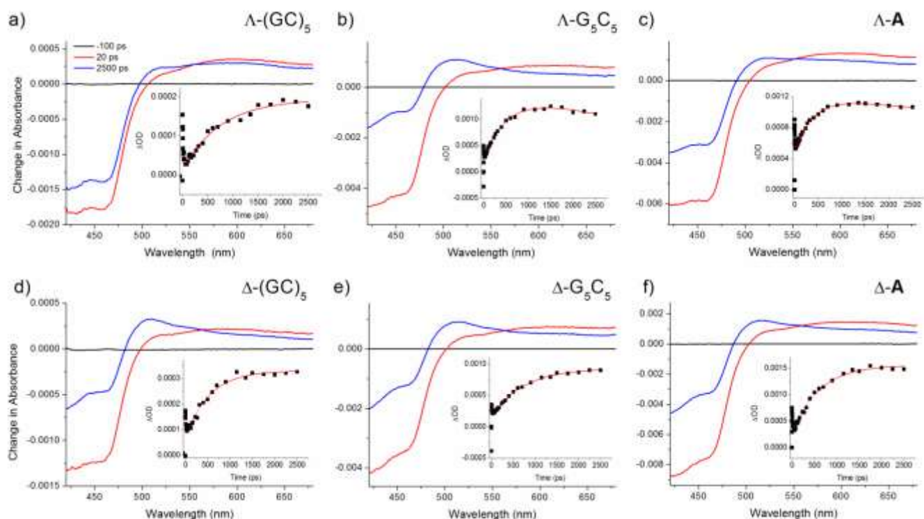
Figure 2. Selected ps-TA spectra (-100 ps, 20 ps, 2500 ps) and associated kinetic fits at 515 nm (inset) for \Lambda -[Ru(TAP) 2 (dppz)] 2+ bound to (a) \{(GC)_5\}_2 (b) \{G_5C_5\}_2 (c) A; and \Delta -[Ru(TAP) 2 (dppz)] 2+ bound to (d) \{(GC)_5\}_2 (e) \{G_5C_5\}_2 (f) A. In each case \lambda_{\text{exc}} = 400 nm, 1 \mu J. [Ru] = 400 \mu M, [ODN] = 500 \mu M duplex in 50 mM phosphate (pH 7) in D 2 O with 50 \mu m pathlength
