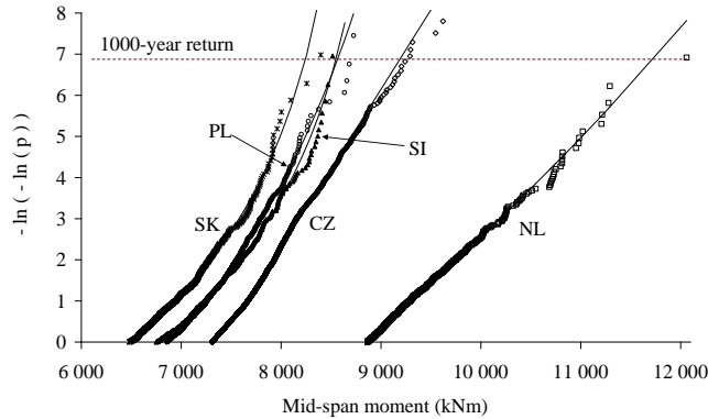
Fig. 4. Annual maximum bending moments from simulation for a 35 m bridge with low lane factors Note: NL=Netherlands, CZ=Czech Republic, SI=Slovenia, PL=Poland, SK=Slovakia
