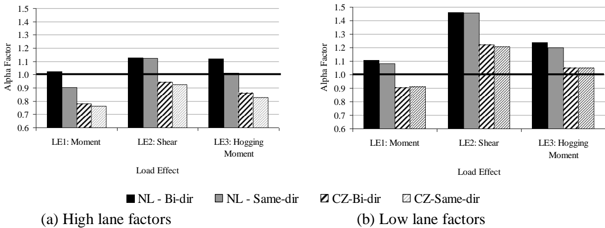
Fig. 6. Comparison of characteristic loads with Eurocode Load Model 1, for bidirectional and two same-direction lanes of traffic.
