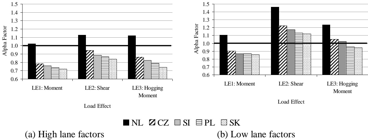
Fig. 5. Comparison of characteristic loads with Eurocode Load Model 1, bidirectional traffic. Note: NL=Netherlands, CZ=Czech Republic, SI=Slovenia, PL=Poland, SK=Slovakia
