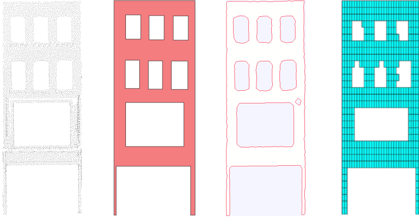
a) Point clouds of the building façade b) Solid models from Kubit software c) Solid models from Geomagic software d) Octree representation using Hinks et al. [50]
