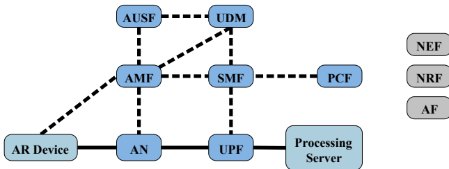
Fig. 9: Architectural components of L5GO to serve the AR use case
