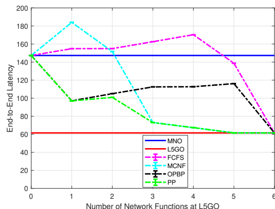
Fig. 25: Average packet latency of sensor networks use case
