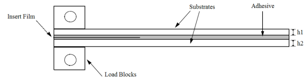
Figure 1: Specimen geometries for DCB ( h_1:h_2 = 1:1 ) & ADCB ( h_1:h_2 = 2:1 )
