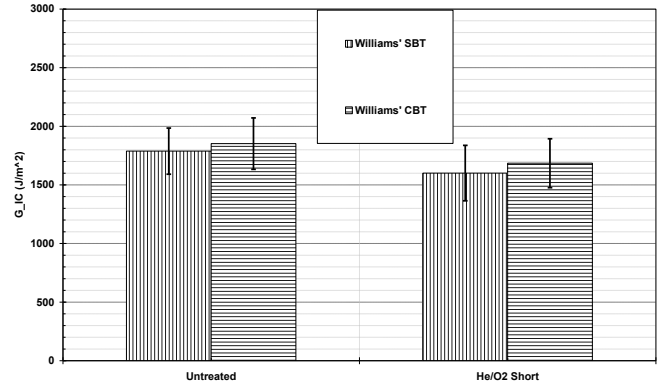
Figure 4: Mean propagation values of G_{IC} ADCB tests.
