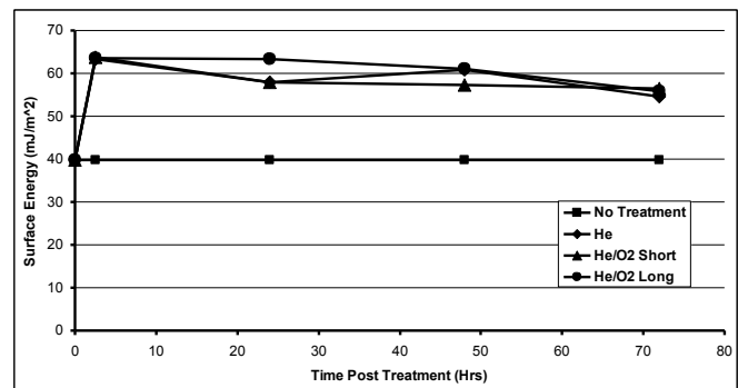
Figure 2: Surface energy versus time post treatment for plasma treatments detailed in Tab. 1.
