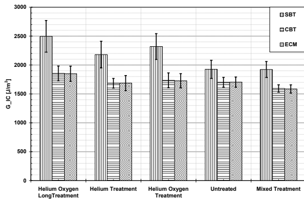
Figure 3: Mean propagation values of G_{IC} DCB tests.
