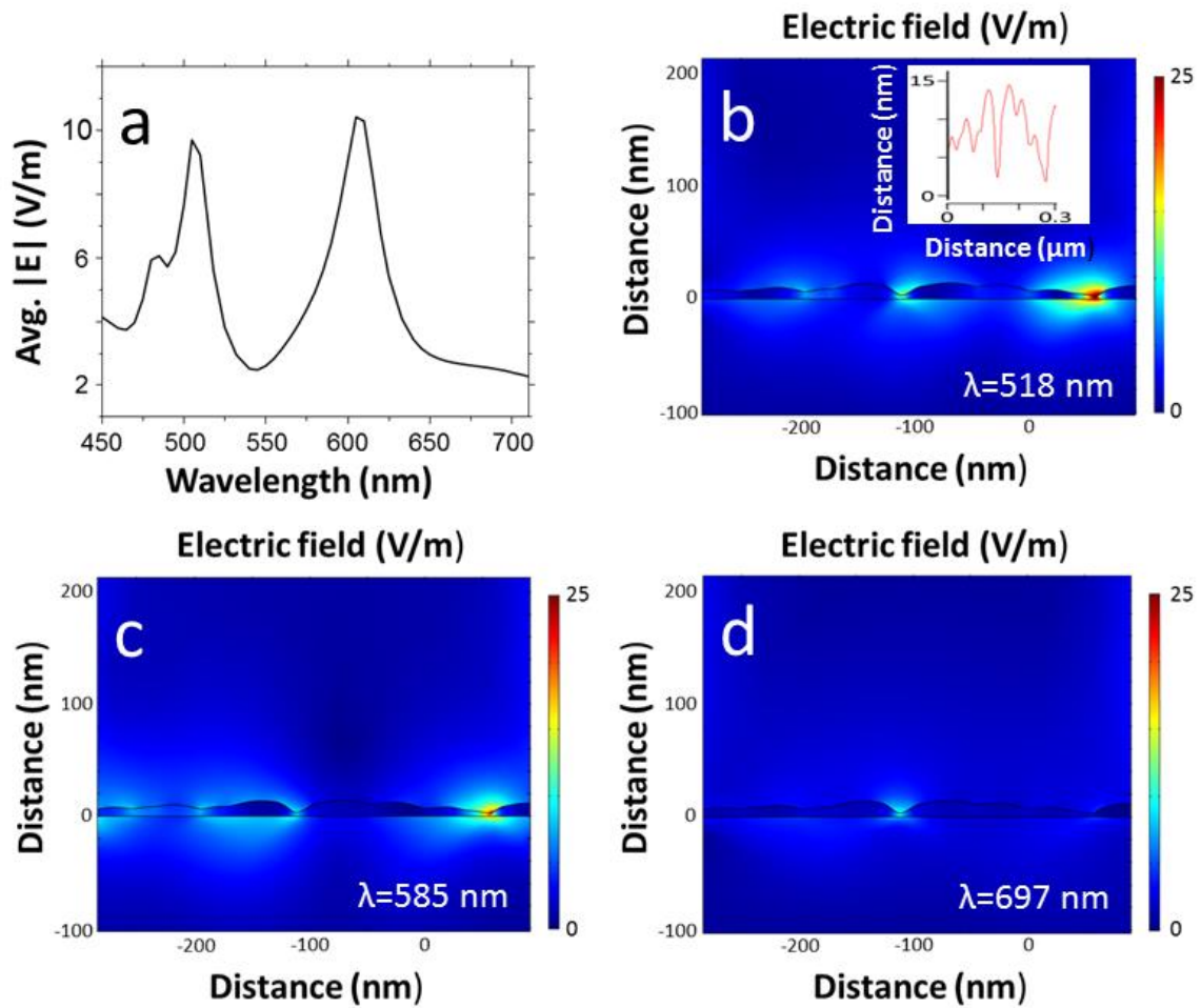
Figure 4. a) Shows the electric field measured at the bottom of the nanopattern spacing at different excitation wavelengths. b), c) and d) show the electric field distribution around a deep nanoparticle spacing along the PPLN silver nanopattern at wavelengths at which the scattered Raman signal from 4-ABT was detected for excitation wavelengths b) \lambda_{\text{ext}}=473 \text{ nm} , c) \lambda_{\text{ext}}=532 \text{ nm} and d) \lambda_{\text{ext}}=633 \text{ nm} . Inset in figure. 4b shows the AFM line profile obtained for the PPLN silver structure used in the COMSOL calculations.
