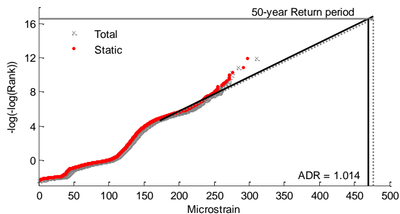
Fig. 5. Extrapolating to 50-year value.
