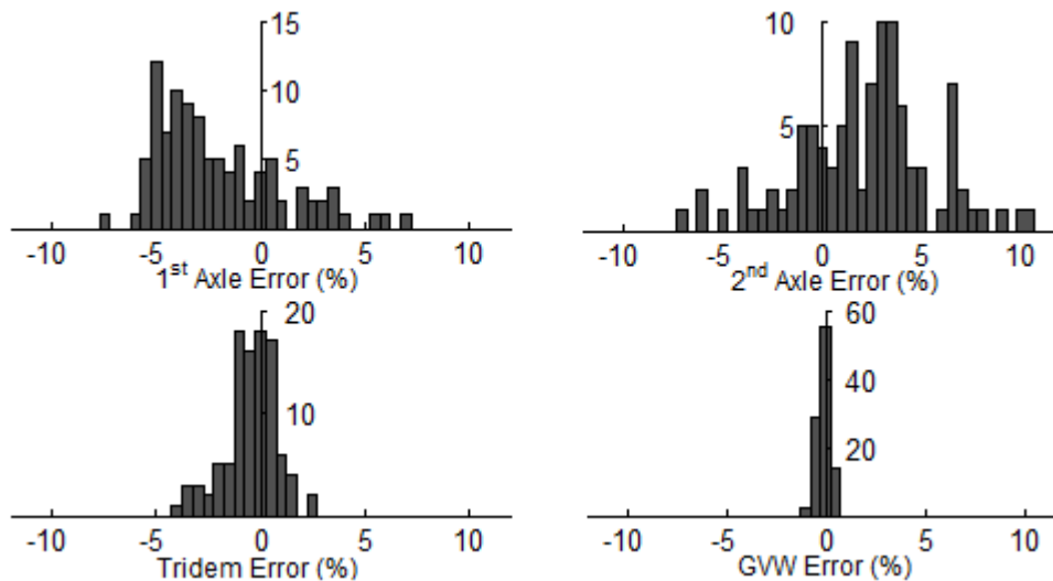
Fig. 9. Bridge WIM Errors.
