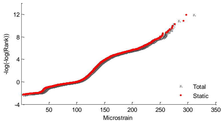
Fig. 4. Gumbel paper plot of measured total and inferred static strains.
