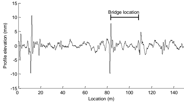
Fig. 6. Measured road profile measured at the bridge in Vransko.
