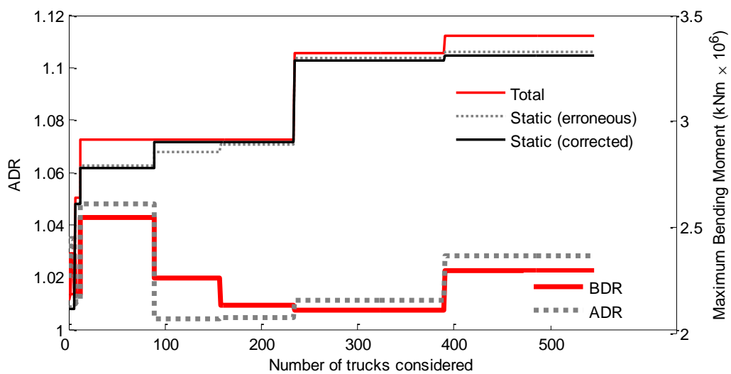
Fig. 10. ADR and BDR.
