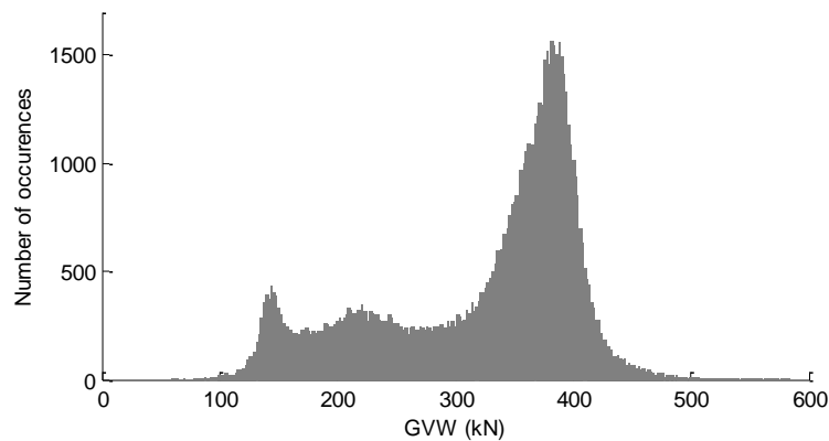
Fig. 2. Histogram of measured GVWs for the 5-axle truck population
