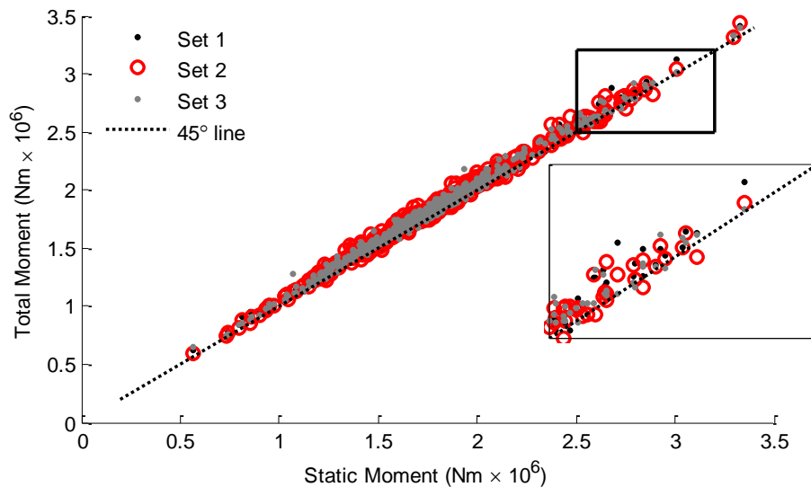
Fig. 7. Results of three simulations.
