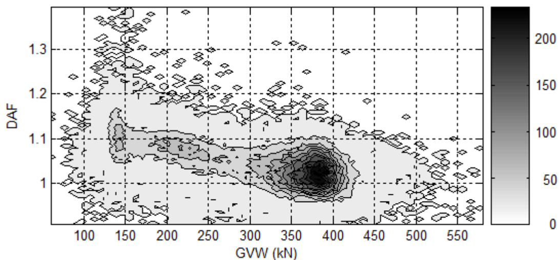
Fig. 3. Contour plot of measured DAF values for mid-span bending moment from the Vranksko site.
