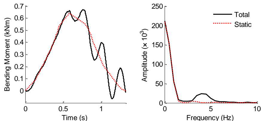
Fig. 1. Time and frequency domain bending moment responses.
