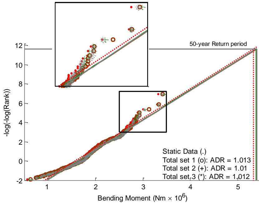
Fig. 8. Results of Extrapolation of Simulation Results.
