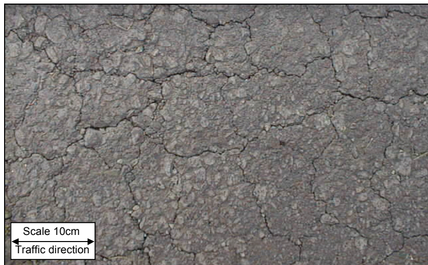
Figure 11. Final crocodile crack pattern observed at 'failure' of road section.
