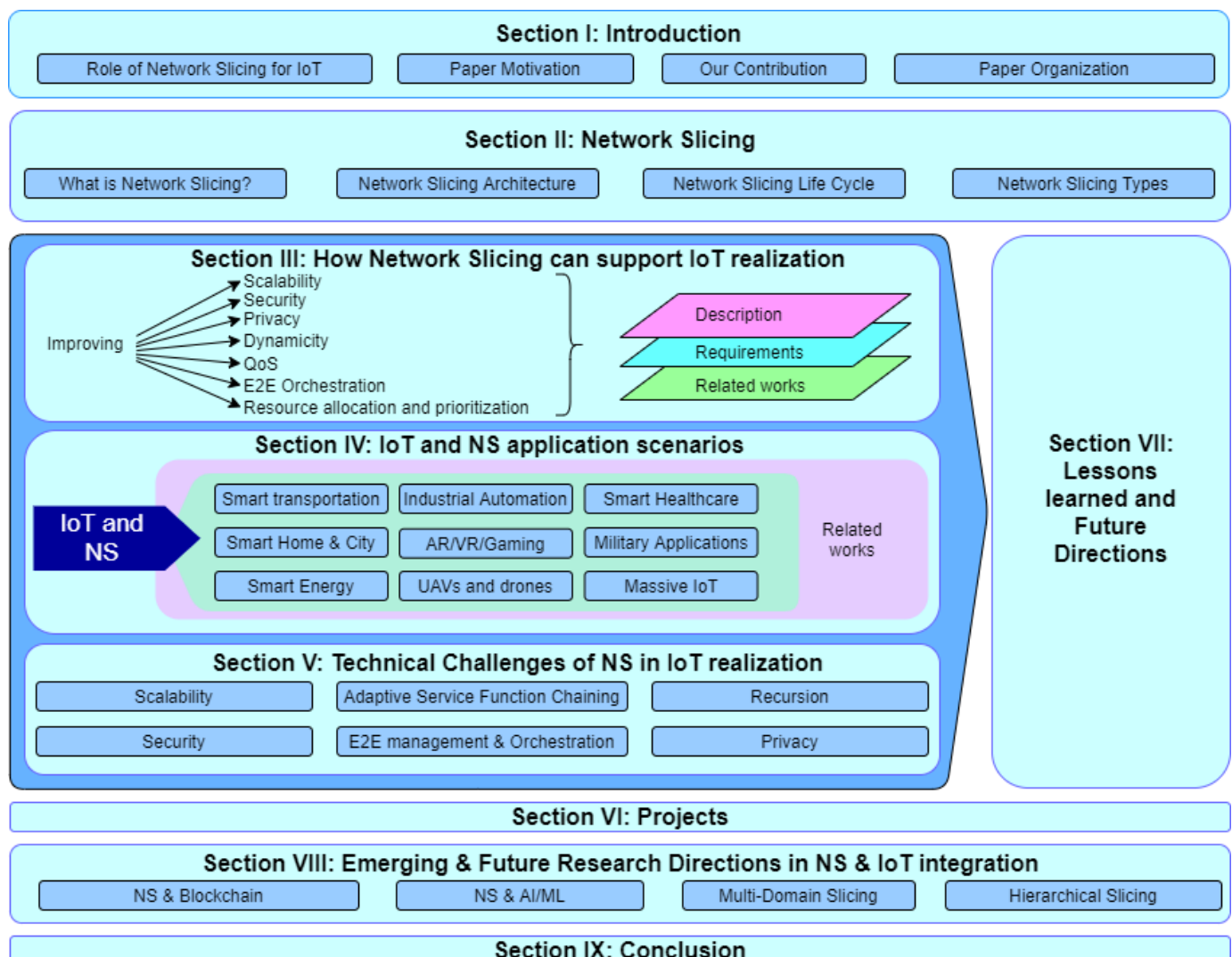
Fig. 3: Paper Organization
